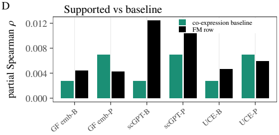
Figure 4. Primary fixed-panel audit under both prespecified confound specifications. (A) Full- confound pooled rows and the same-edge co-expression baseline; labels give BH-adjusted q_M and q_D for FM rows and uncorrected p_M, p_D for the baseline. (B) Non-degree co-primary rows; no row is supported by both nulls. (C) Full-confound q_M versus q_D ; support requires both coordinates below 0.05. (D) Each supported positive row compared with its own-tissue co-expression baseline.
