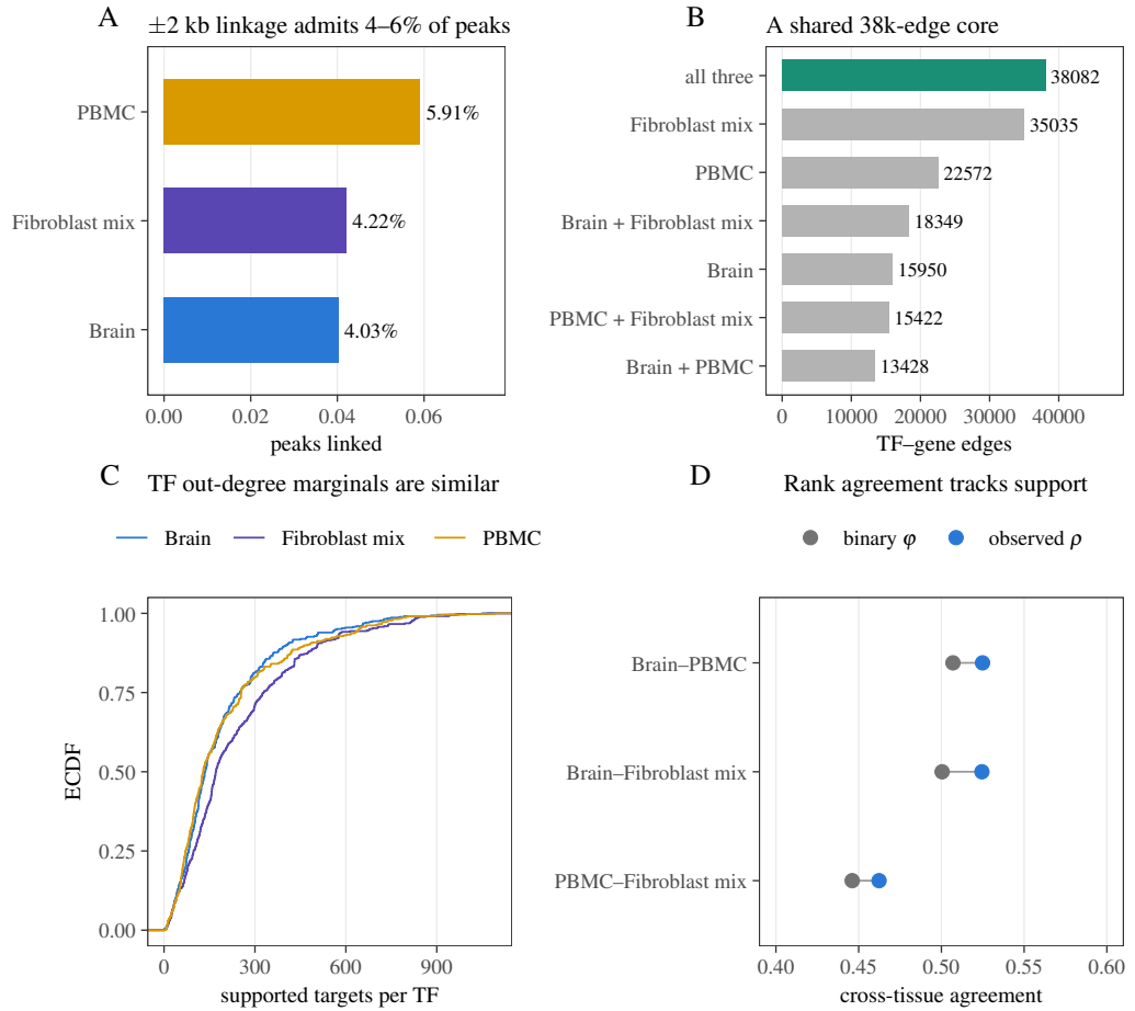
Figure 11. Third-tissue transfer of the proxy construct. (A) Fraction of each dataset’s peaks admitted by the \pm 2 kb linkage window (relevant over total peaks). (B) Overlap of supported (nonzero) non-self TF–gene edges across the three consensus proxies; the green bar is the 38,082-edge core present in all three. (C) Empirical CDF of TF out-degree (supported targets per TF) per tissue. (D) Observed cross-tissue Spearman \rho versus binary-support \phi for the three tissue pairs.
