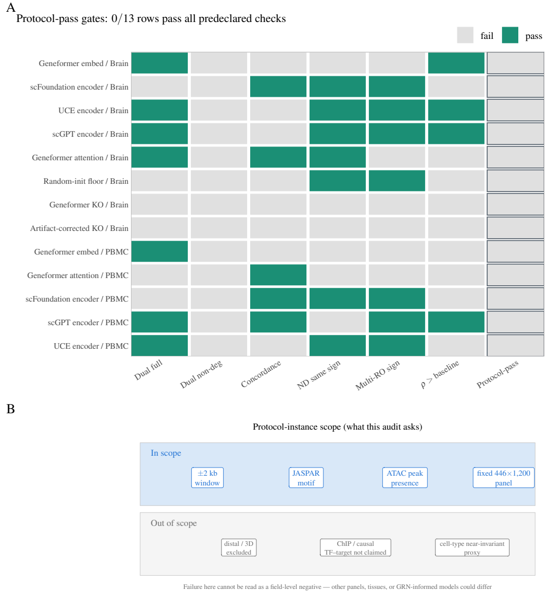
Figure 12. Protocol-pass and instance scope. (A) Binary gate heatmap for the thirteen pooled FM/readout rows (aqua pass, grey fail), companion to Table 4. Protocol-pass is the conjunction column (outlined); no row passes (0/13). (B) Protocol-instance scope card: the audit scores motif matches in \pm 2 kb-linked ATAC peaks on a fixed panel. Distal/3D structure and ChIP-derived causal TF–target maps are out of scope; the proxy is cell-type near-invariant on this panel. Failure to support a global capability claim therefore cannot be read as a field-level negative (Sec. 2.1).
