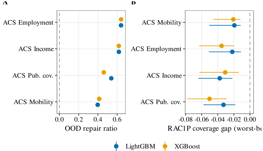
Figure 7: Generalization to a TableShift-class benchmark (Folktables/ACS, leave-states-out spatial OOD). A. OOD abstention repair ratio per ACS task (XGBoost vs. LightGBM, 400-bootstrap CIs); the repair ratio is the fractional reduction in integrated selective risk vs. random deferral, so positive ratios (CI excluding 0) mean uncertainty abstention beats random deferral, replicating on 4/4 tasks for both GBMs. B. RAC1P race-subgroup conformal coverage gap (worst–best); the OOD reliability gap manifests as a negative subgroup coverage gap (CI excluding 0 on 4/4 for both GBMs) rather than a marginal-AURC blow-up.
