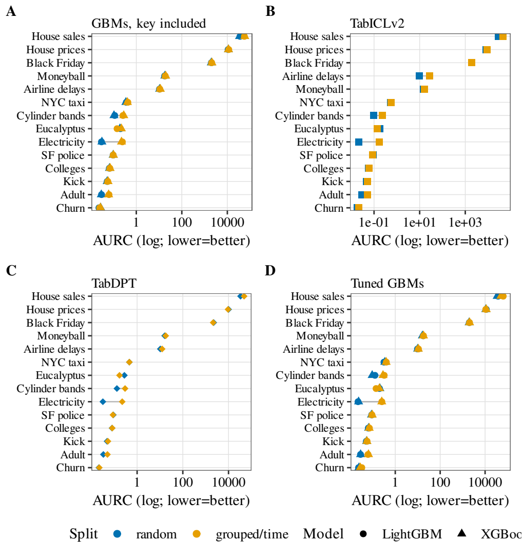
Figure 2: Per-dataset risk-coverage AUC under random vs. grouped/time split, shown as paired points on a log-scaled AUC axis (classification and regression AUC span several orders of magnitude). A GBMs with the group key included; B TabICLv2; C TabDPT; D tuned GBM baseline. Grouped/time points sit to the right of random on most datasets (higher AUC, worse selective risk).
