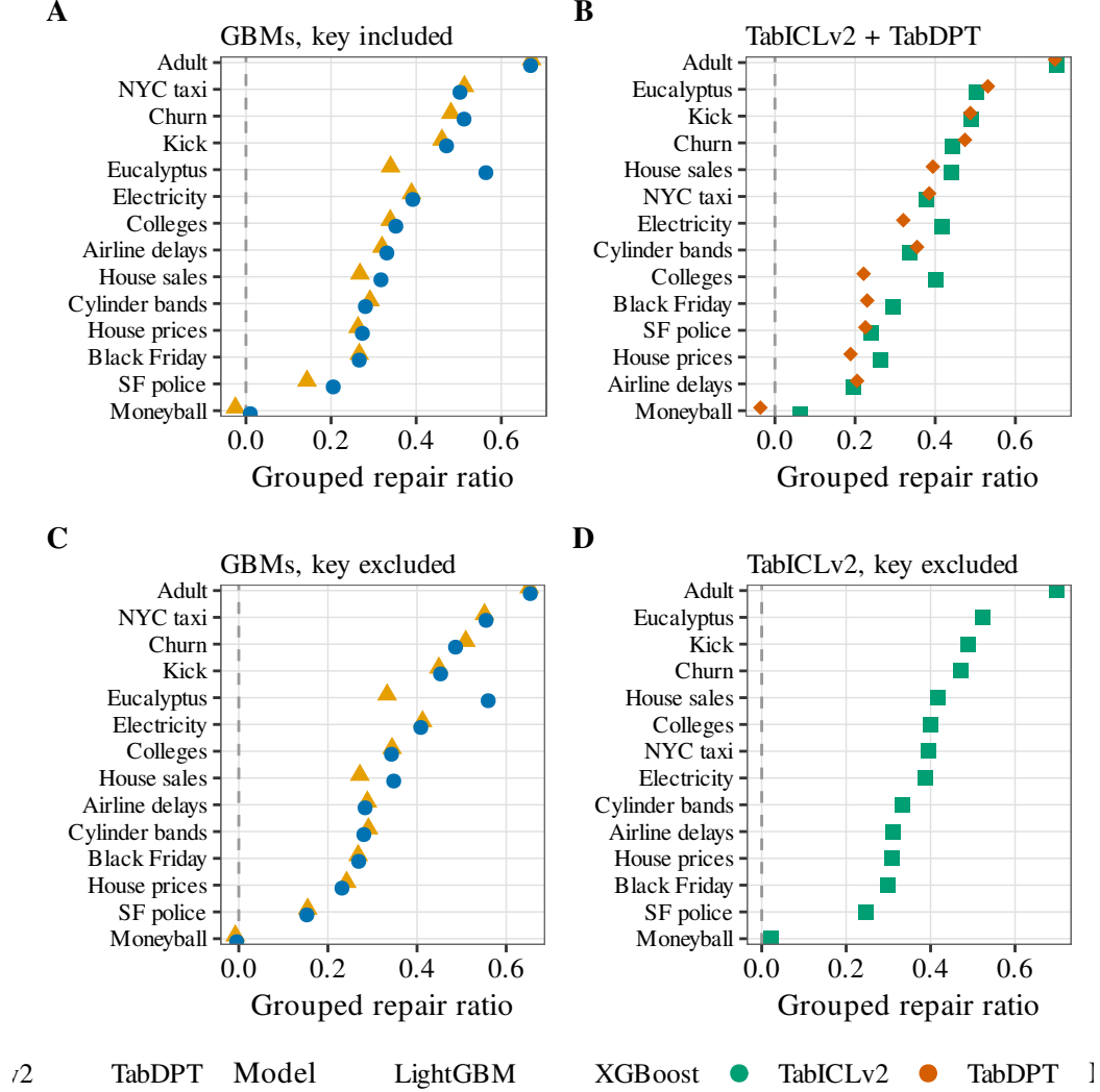
Figure 3: Uncertainty-ranked abstention beats random deferral under the grouped split. Each point is one dataset’s repair ratio—the share of the random-deferral selective-risk AURC that abstention removes—with datasets ordered by ratio; points right of the dashed zero line improve on random deferral. A GBMs, key included; B TabICLv2 and TabDPT; C GBMs, key excluded; D TabICLv2, key excluded.
