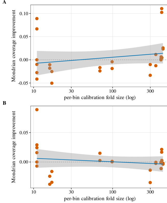
Figure 6: Why Mondrian conformal fails, and why that explanation is key-dependent (reconciled RNG). A Key-included: per-bin calibration fold size predicts Mondrian’s coverage improvement (Spearman \rho = 0.50 , CI excluding zero; clean-threshold separation bacc = 0.854, p = 0.0011 )—the mechanism passes the preregistered bar. B Key-excluded: dropping the group key from the model features collapses the relationship ( \rho = -0.12 , no significant predictors, threshold bacc = 0.548), flipping the preregistered verdict to KILL. The calibration-size mechanism is real but key-dependent—the paper’s protocol-sensitivity finding applied to its own mechanism.
