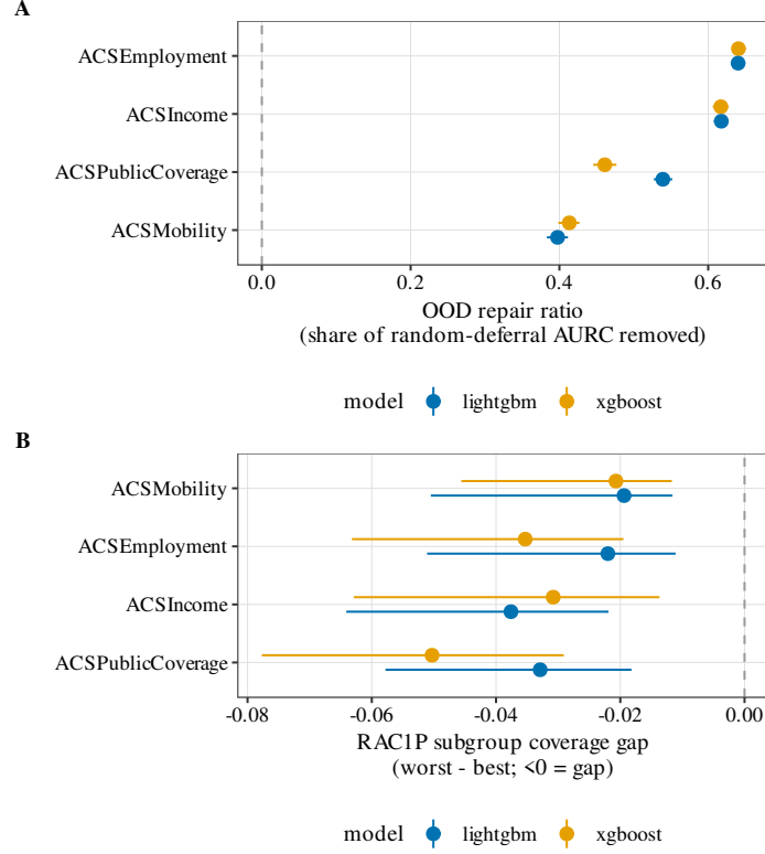
Figure 7: Generalization to a TableShift-class benchmark (Folktables/ACS, leave-states-out spatial OOD). A OOD abstention repair ratio per ACS task (XGBoost vs. LightGBM, 400-bootstrap CIs); the repair ratio is the fractional reduction in integrated selective risk vs. random deferral, so positive ratios (CI excluding 0) mean uncertainty abstention beats random deferral, replicating on 4/4 tasks for both GBMs. B RAC1P race-subgroup conformal coverage gap (worst–best); the OOD reliability gap manifests as a negative subgroup coverage gap (CI excluding 0 on 4/4 for both GBMs) rather than a marginal-AURC blow-up.
