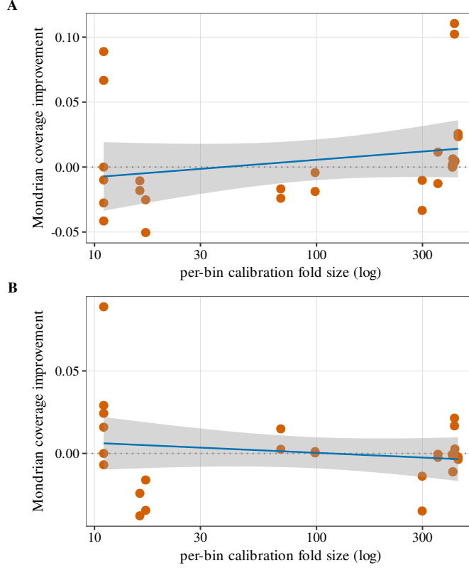
Fig. 6 Why Mondrian conformal fails, and why that explanation is key-dependent (reconciled RNG). A Key-included: per-bin calibration fold size predicts Mondrian’s coverage improvement (Spearman \rho = 0.50 , CI excluding zero; clean-threshold separation \text{bacc} = 0.854 , p = 0.0011 )—the mechanism passes the preregistered bar. B Key-excluded: dropping the group key from the model features collapses the relationship ( \rho = -0.12 , no significant predictors, threshold \text{bacc} = 0.548 ), flipping the preregistered verdict to KILL. The calibration-size mechanism is real but key-dependent—the paper’s protocol-sensitivity finding applied to its own mechanism.
