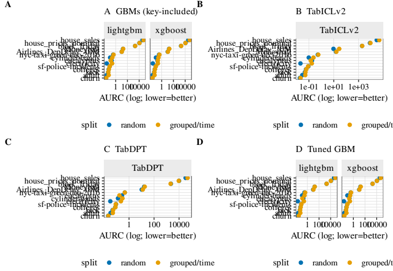
Fig. 2 Per-dataset risk-coverage AURC under random vs. grouped/time split, shown as paired points on a log-scaled AURC axis (per-dataset AURC spans several orders of magnitude across classification and regression tasks, so a shared linear axis renders most datasets illegible): grouped splits degrade reliability.
