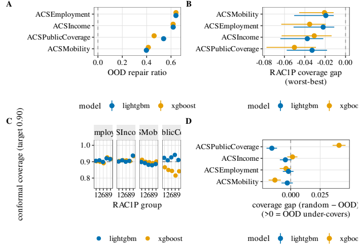
Fig. 7 Generalization to a TableShift-class benchmark (Folktables/ACS, leave-states-out spatial OOD). A OOD abstention repair ratio per ACS task (XGBoost vs. LightGBM, 400-bootstrap CIs); the repair ratio is the fractional reduction in integrated selective risk vs. random deferral, so positive ratios (CI excluding 0) mean uncertainty abstention beats random deferral, replicating on 4/4 tasks for both GBMs. B RAC1P race-subgroup conformal coverage gap (worst–best); the OOD reliability gap manifests as a negative subgroup coverage gap (CI excluding 0 on 4/4 for both GBMs) rather than a marginal-AURC blow-up.
