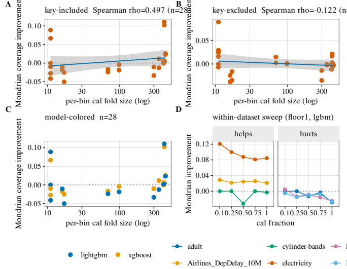
Fig. 6 Why Mondrian conformal fails, and why that explanation is key-dependent (reconciled RNG). A Key-included: per-bin calibration fold size predicts Mondrian’s coverage improvement (Spearman \rho = 0.50 , CI excluding zero; clean-threshold separation \text{bacc} = 0.854 , p = 0.0011 )—the mechanism passes the preregistered bar. B Key-excluded: dropping the group key from the model features collapses the relationship ( \rho = -0.12 , no significant predictors, threshold \text{bacc} = 0.548 ), flipping the preregistered verdict to KILL. The calibration-size mechanism is real but key-dependent—the paper’s protocol-sensitivity finding applied to its own mechanism.
