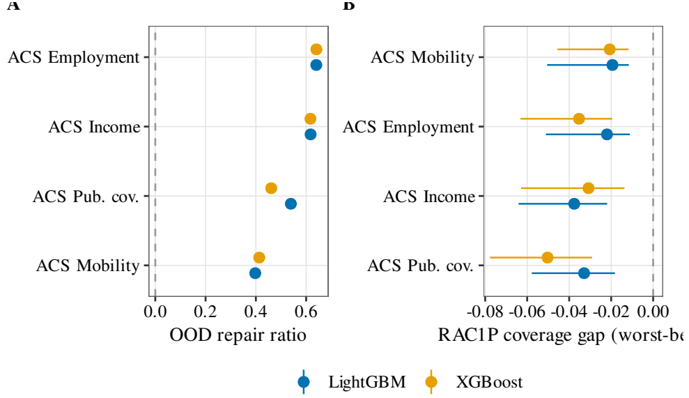
Fig. 7 Generalization to a TableShift-class benchmark (Folktables/ACS, leave-states-out spatial OOD). A. OOD abstention repair ratio per ACS task (XGBoost vs. LightGBM, 400-bootstrap CIs); the repair ratio is the fractional reduction in integrated selective risk vs. random deferral, so positive ratios (CI excluding 0) mean uncertainty abstention beats random deferral, replicating on 4/4 tasks for both GBMs. B. RAC1P race-subgroup conformal coverage gap (worst–best); the OOD reliability gap manifests as a negative subgroup coverage gap (CI excluding 0 on 4/4 for both GBMs) rather than a marginal-AURC blow-up.
