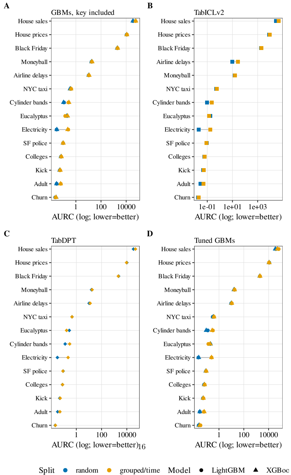
Fig. 2 Per-dataset risk-coverage AURC under random vs. grouped/time split, shown as paired points on a log-scaled AURC axis (classification and regression AURC span several orders of magnitude). A GBMs with the group key included; B TabICLv2; C TabDPT; D tuned GBM baseline. Grouped/time points sit to the right of random on most datasets (higher AURC, worse selective risk).
