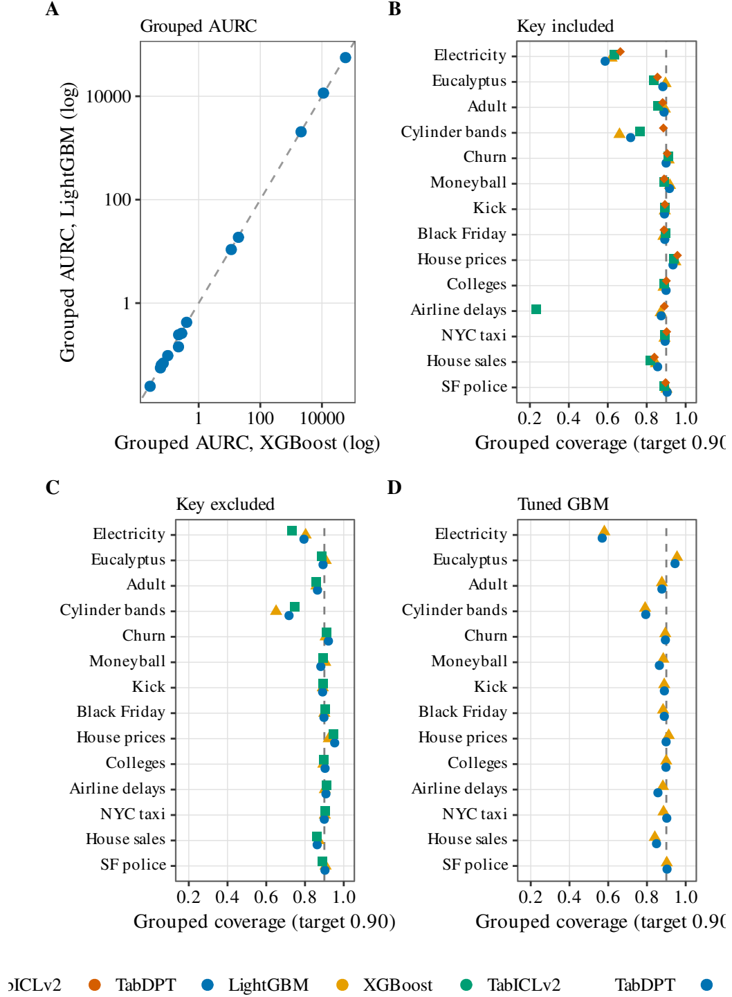
Figure 4: Model-agnosticism across four configurations spanning three architecture families. A. Grouped AURC for XGBoost versus LightGBM on all 14 datasets (log-log; points near the diagonal show the two gradient-boosted models behave near-identically). B. Split-conformal grouped coverage with the group key included, all four configurations;
