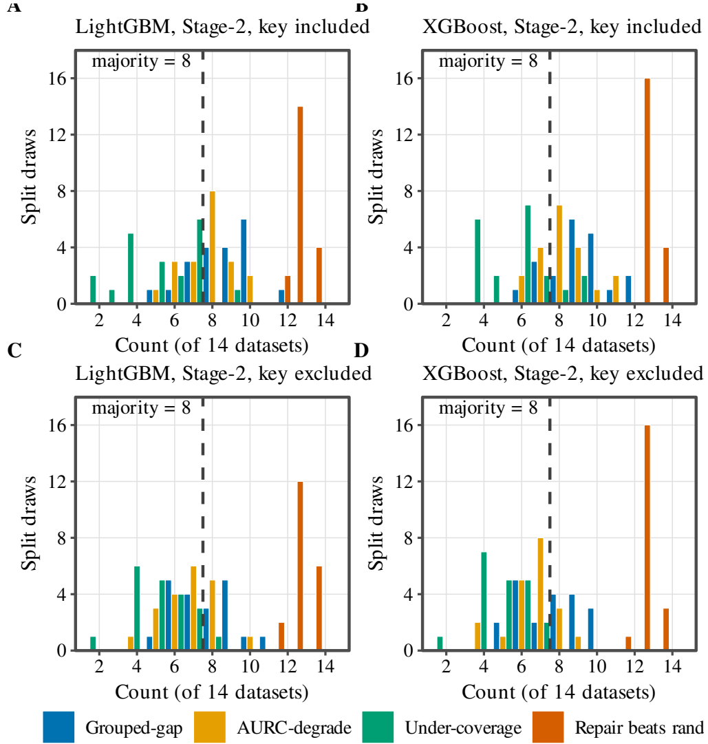
Figure 5: Split-realization fragility of the four headline counts over K repeated grouped-split draws (count out of 14 datasets; dashed line at the preregistered majority threshold of 8). A. LightGBM, Stage-2, key included. B. XGBoost, Stage-2, key included. C. LightGBM, Stage-2, key excluded. D. XGBoost, Stage-2, key excluded. The grouped-gap count straddles the threshold—majority-robust in 75% of LightGBM key-included draws (Stage-2 XGBoost 80%; combined range 75–83%)—AURC-degrade likewise straddles it, and under-coverage falls below it; only repair-beats-random sits at the top and never drops below the threshold (100% of draws). This is why we treat the repair, not the degradation-side counts, as the load-bearing finding.
