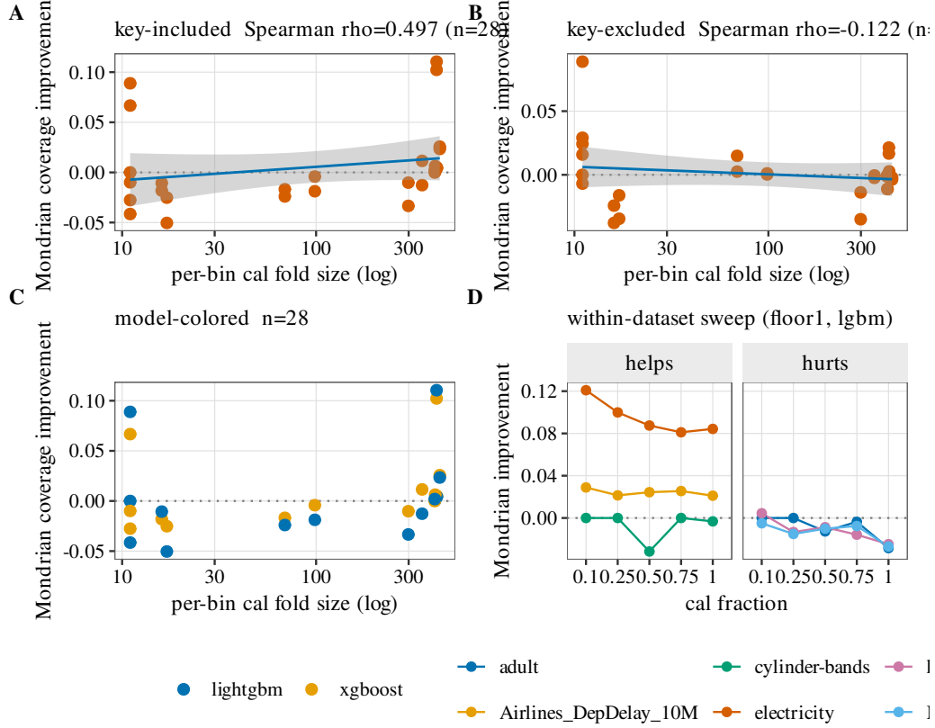
Figure 7: Why Mondrian conformal fails, and why that explanation is key-dependent (reconciled RNG). A. Key-included: per-bin calibration fold size predicts Mondrian’s coverage improvement (Spearman \rho = 0.50 , CI excluding zero; clean-threshold separation \text{bacc} = 0.854 , p = 0.0011 )—the mechanism passes the preregistered bar. B. Key-excluded: dropping the group key from the model features collapses the relationship ( \rho = -0.12 , no significant predictors, threshold \text{bacc} = 0.548 ), flipping the preregistered verdict to KILL. The calibration-size mechanism is real but key-dependent—the paper’s protocol-sensitivity finding applied to its own mechanism. C. Model-colored view of all 28 (dataset \times model) rows from the key-included diagnostic. D. Designed within-dataset sweep (floor1 rule, LightGBM): calibration fraction vs. improvement, grouped by whether Mondrian helps or hurts the dataset.
