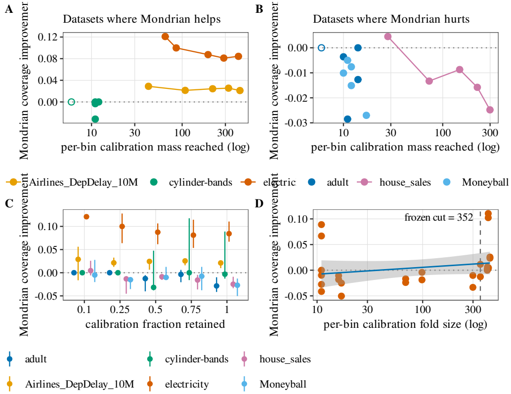
Figure 6: The designed within-dataset calibration sweep (post-freeze exploratory): dose-response does not hold within a dataset. A. Three datasets where Mondrian helps: improvement vs. achieved per-bin calibration mass (log axis), three seeds. B. Three where it hurts: adding mass makes Mondrian worse (median Spearman -0.51 , negative in 5/6 series). C. Seed envelope per dataset and fraction (min-max over three carve-out seeds). D. Full-calibration cross-section reproducing the frozen diagnostic cut at 352 (dashed): the between-dataset regularity, which the within-dataset sweep shows is not a calibration-budget lever. From the frozen planning-sweep record.
