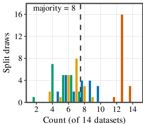
D XGBoost, Stage-2, key excluded
