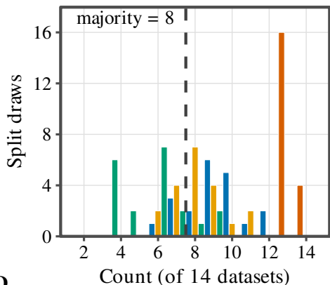
D XGBoost, Stage-2, key excluded
