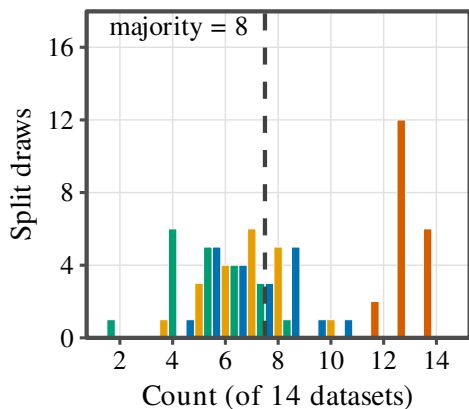
C LightGBM, Stage-2, key excluded
