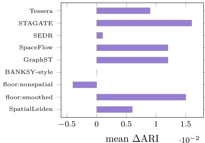
Figure 9: The law survives the author-recommended backend (real R mclust): published versus mclust-backend advantage stays close to the diagonal for most datasets (a; a few, such as IMC, move more), and the fairer backend shifts every method’s mean ARI by \leq 0.016 (b).
