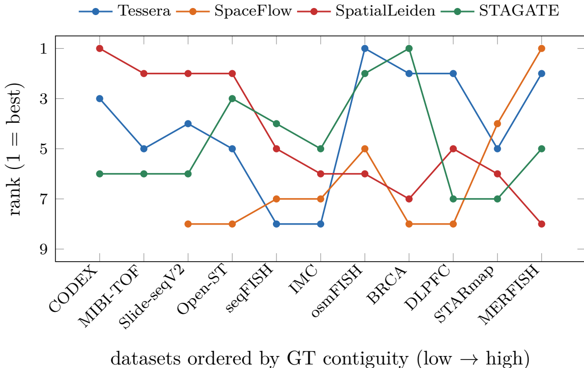
Figure 2: Per-method rank versus GT contiguity. Method–task fit is method-specific: SpatialLeiden’s profile is inverted (wins low-contiguity datasets, last on high-contiguity MERFISH).
