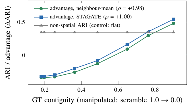
Fig. 7: Controlled mechanism: with the expression signal held fixed (flat grey control), spatial-prior advantage rises with manipulated contiguity and flips sign, giving causal evidence for the law.
