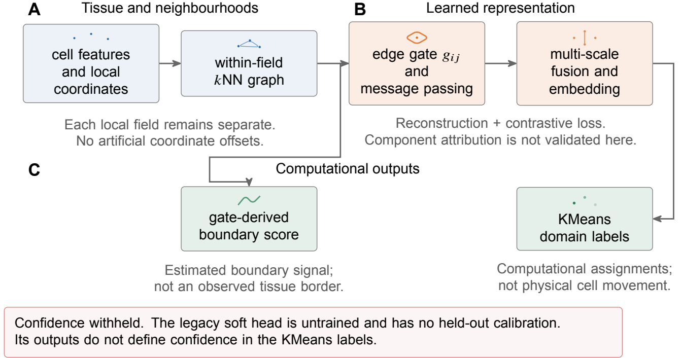
Figure 6: Implemented candidate pipeline and its evidence boundary. Local tissue coordinates define within-field neighbours in the repaired graph; features pass through a learned gate, message passing and multi-scale fusion. The embedding supplies KMeans domain labels and a feature-reconstruction objective; gate-derived boundary scores are computational estimates, not observed histological borders. The contrastive objective uses graph neighbours as positives and sampled nodes as negatives. A separate legacy soft head has no training-loss or held-out calibration step and does not supply validated confidence in KMeans labels; that output is withheld. Field-aware graph support does not establish a corrected external-method benchmark.
