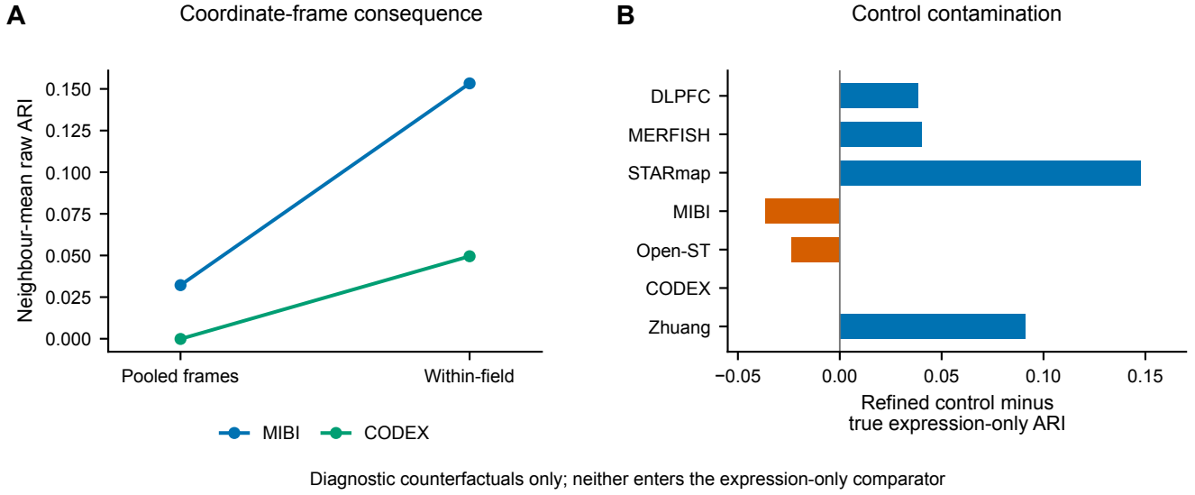
Figure 2: Direct consequences of two protocol errors, evaluated on the same inputs and seeds as the repaired analysis. (A) Three-seed mean neighbour-mean PCA–KMeans ARI with pooled local coordinates versus within-field coordinates for MIBI and CODEX. All other fitting settings are fixed. (B) Change in the nominal control’s ARI if its expression-only labels are spatially refined. These diagnostic arms are not eligible controls, and no maximum across them is used.
