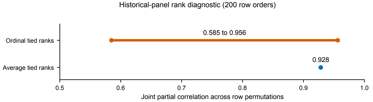
Figure 4: Tie-handling diagnostic on the unchanged historical eleven-object panel. Across 200 row permutations, ordinal ranks assigned to tied class counts, feature dimensions and modalities change the joint partial correlation from 0.585 to 0.956. Average ranks preserve equal values and return 0.928 for every ordering to numerical precision. The horizontal span is a computational order-sensitivity range, not a confidence interval. Correcting this algorithm does not repair the historical coordinates or control and is not evidence of an independent biological mechanism.
