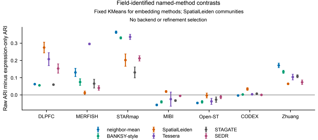
Figure 1: Each named spatial method minus the genuinely expression-only comparator on the same cells and original seed identities. Dots are three-seed means; whiskers are the sample SD of the paired seed differences, not tissue-level confidence intervals. KMeans and raw assignments are fixed, so no true-label winner or refinement selection defines the contrast. Missing external methods are not imputed or included in an oracle maximum.
