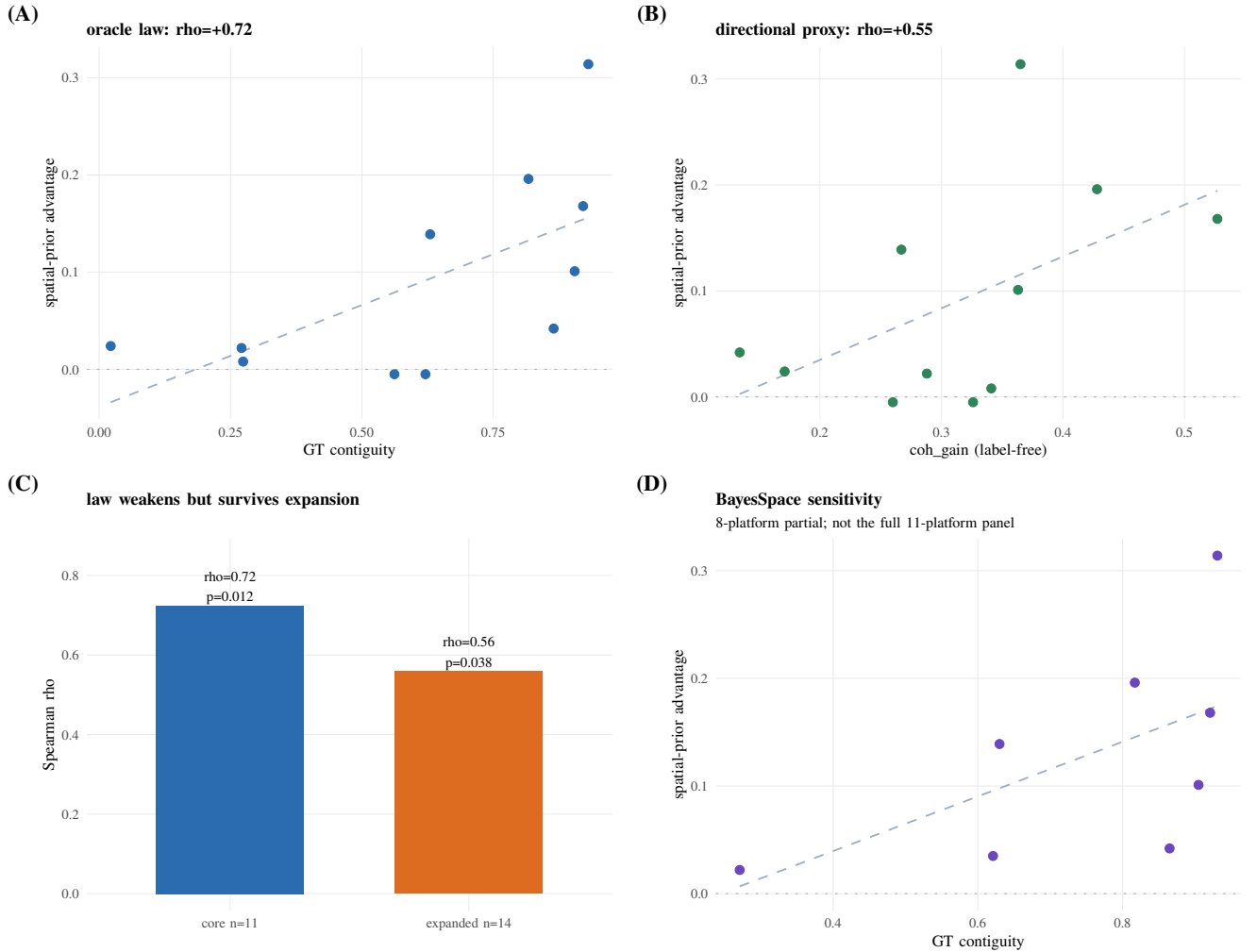
Fig. 4: (a) The headline law: spatial-prior advantage versus GT spatial contiguity (oracle), \rho = +0.72 . (b) The same trend recovered by the label-free coh_gain proxy, \rho = +0.55 , the rule applied without labels.
