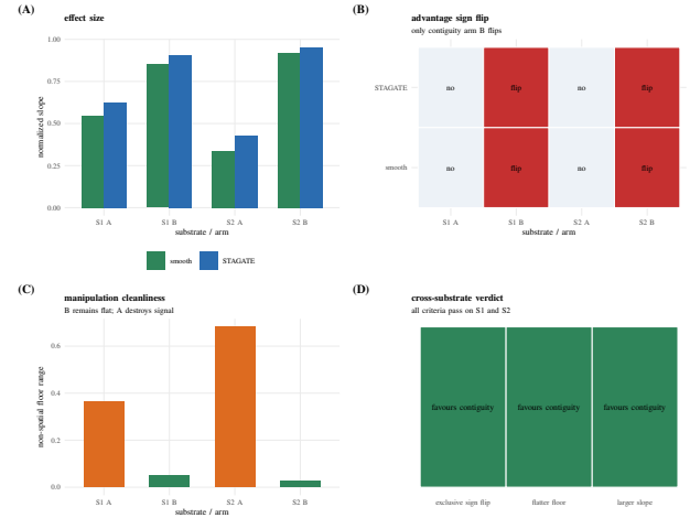
Fig. 7: Controlled mechanism: with the expression signal held fixed (flat grey control), spatial-prior advantage rises with manipulated contiguity and flips sign, giving causal evidence for the law.
