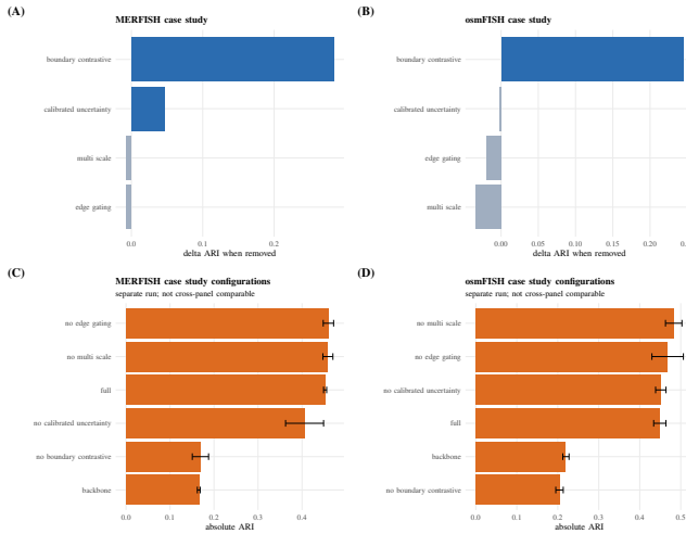
Fig. 11: Component ablation of the candidate method on the two datasets where it is competitive (3 seeds): the ARI drop when each component is removed (positive = the component contributes). Only the boundary-contrastive loss matters; the headline anti-over-smoothing edge gate and multi-scale fusion are neutral-to-harmful, so the model’s gain over a plain backbone is the contrastive loss alone. These absolute ARIs come from a separate two-dataset case-study run and are not directly comparable with the cross-dataset benchmark panels.
