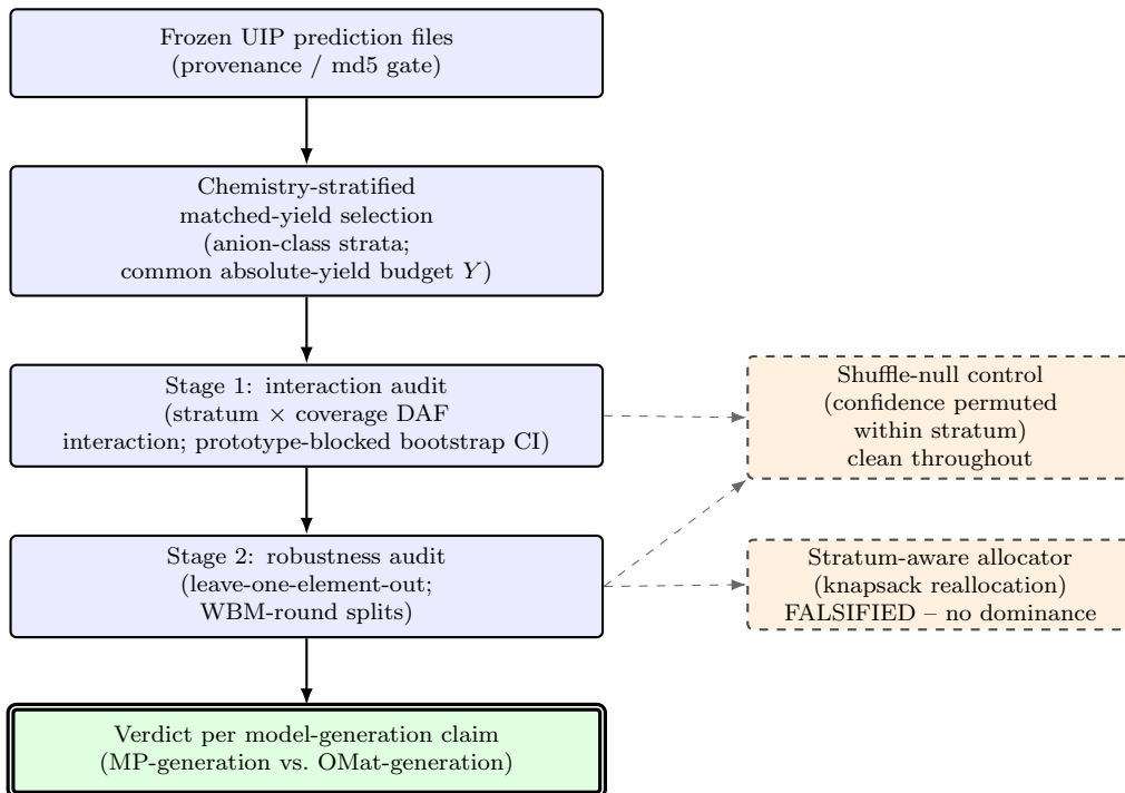
Figure 1: The matched-yield reliability-audit protocol. Frozen, provenance/md5-gated UIP prediction files feed a chemistry-stratified matched-yield selection (anion-class strata, common absolute-yield budget Y ), which is audited in two stages — the Stage 1 stratum \times coverage DAF interaction and the Stage 2 leave-one-element-out / WBM-round robustness gates — to a verdict per model-generation claim. Two built-in controls (dashed) guard the audit: a shuffle-null that stays clean throughout, and a stratum-aware knapsack allocator that the protocol itself falsified.
