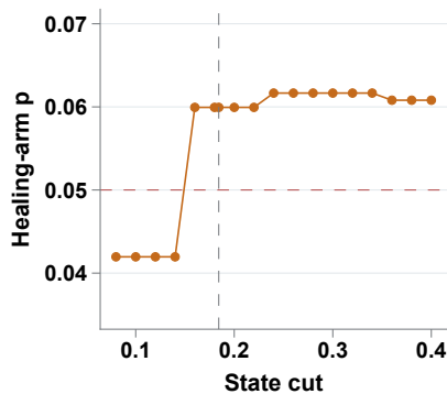
E Structureless input
