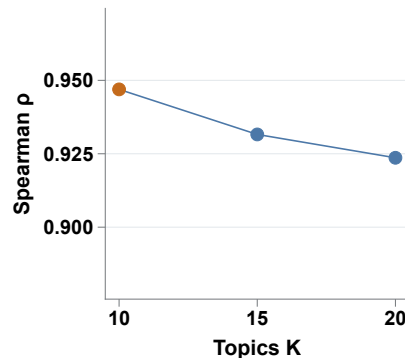
F Null calibration
