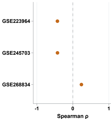
B Detected genes
