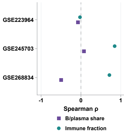
A Immune context
