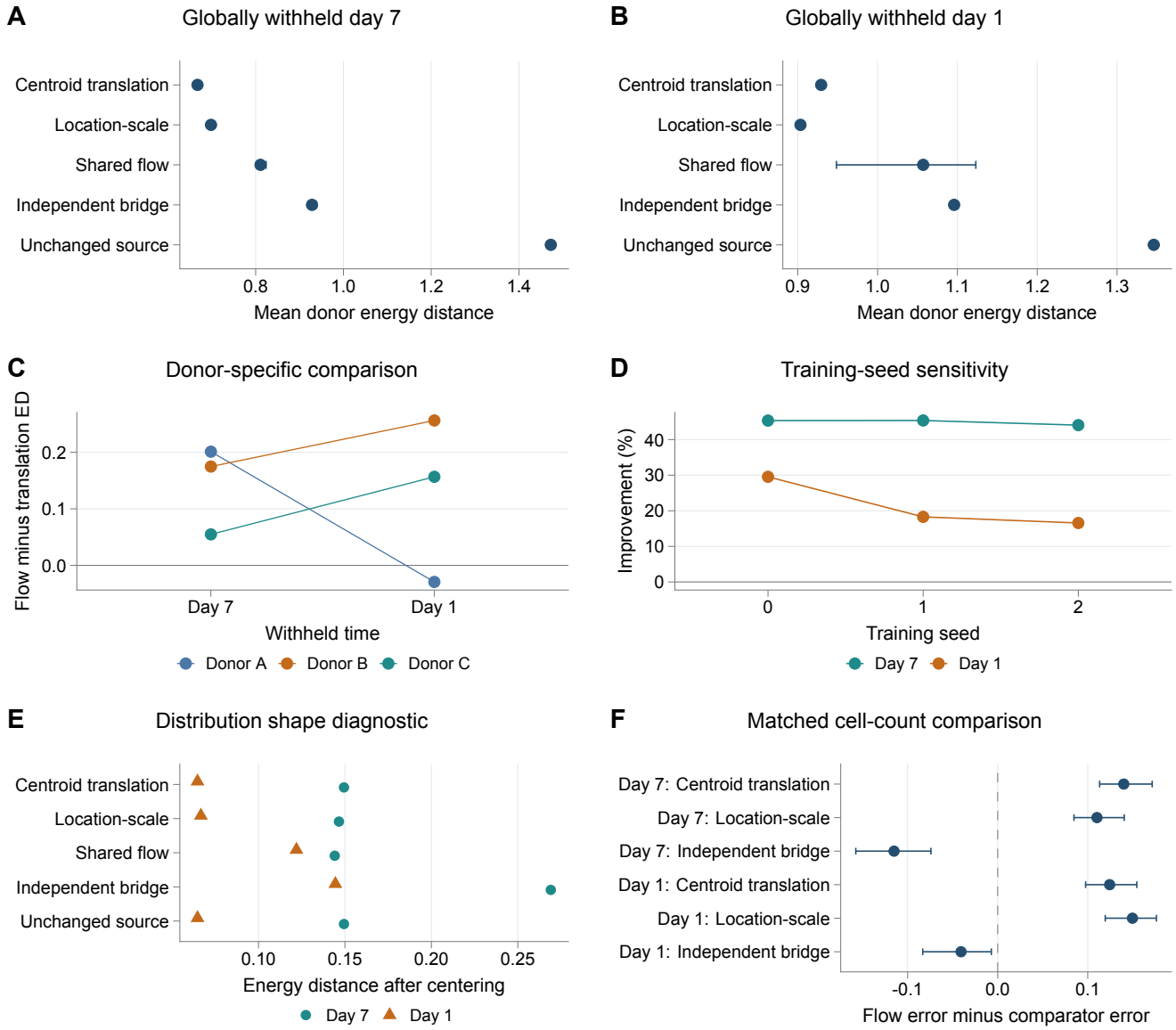
Figure 3. Simple baselines for globally missing times. All methods use the same frozen representation and training exclusions; error averages full-cell empirical energy distances within the three donors. (A) Withheld day 7, predicted from day 1 with day 30 as the observed anchor. (B) Withheld day 1, predicted from intact skin with day 7 as anchor. Points show the three-seed mean error; horizontal ranges show seed minima and maxima, not confidence intervals. Both tasks use the fixed rank-time interpolation fraction one half. (C) Donor-specific seed-averaged field error minus centroid-translation error; positive values favor translation. The later anchor belongs to the same donor, so this is retrospective interpolation rather than source-only donor transfer. (D) Each field seed's improvement over the corresponding unchanged source. Seeds and repeated distance evaluations provide no additional biological replication. (E) Seed- and donor-averaged energy distance after separately centering each distribution; this diagnoses shape without decomposing total error. (F) Mean and full range of flow-minus-comparator errors across 50 paired draws of 200 source and 200 target cells per donor; positive values favor the comparator. Location-scale uses only endpoint means and coordinate standard deviations. Matched draw ranges are not confidence intervals.
