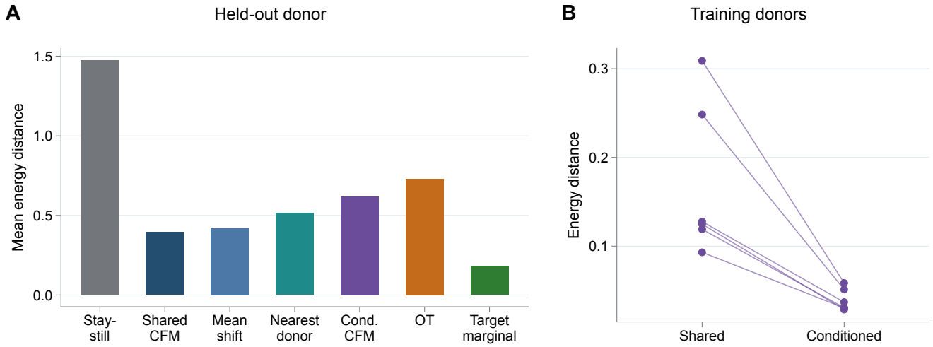
Figure 5. Method comparison across three held-out donors. (A) Bars are equally donor-weighted mean energy distances for unchanged source, five historical predictors and the added matched-particle target marginal. CFM means conditional flow matching; OT is the entropic transport displacement extension. The target marginal assigns equal mass to the two training donors' Wound7 distributions, uses no held-source expression, and averages 50 draws under the original target samples and scaling. Its mean error is 0.1818 versus 0.3947 for historical shared CFM, but PWH28 favors the field. All historical predictive methods exceeded the single split-half gain reference in 3/3 folds; this descriptive criterion is not a significance test or population ranking. (B) Lines connect shared and conditioned errors for six training-donor comparisons (two retained donors in each of three fits). Conditioning improves all six. These comparisons share donors and do not measure unseen-donor transfer. Neither panel shows uncertainty intervals.
