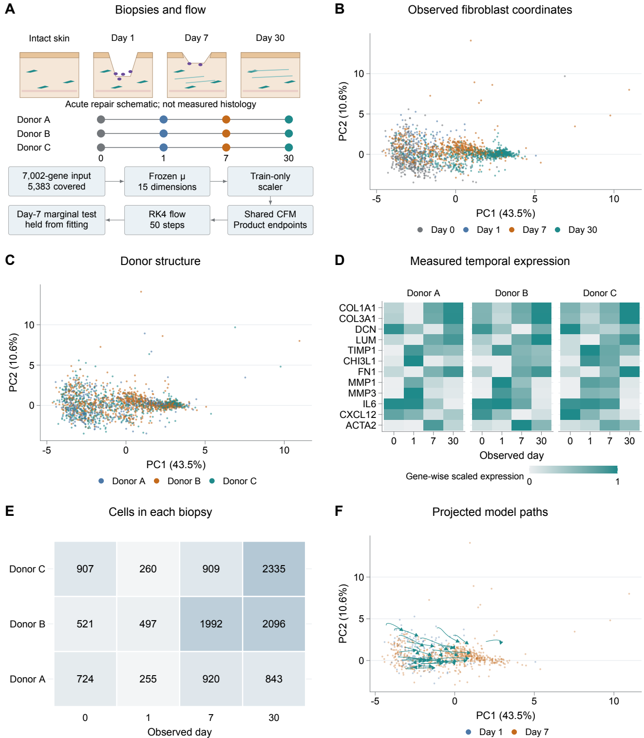
Figure 1. Acute-wound sampling and frozen-coordinate flow. (A) Conceptual repair, not measured histology or closure time, and repeated biopsies of three healthy donors at days 0, 1, 7 and 30. The lower route starts with 7,002-gene proportions: 5,383 panel genes are covered and the remainder zero-filled. A frozen 15-dimensional encoder mean \mu is scaled using training cells only. A shared conditional-flow-matching (CFM) field learns from independently sampled product-coupled endpoints; 50-step RK4 predicts the day-7 marginal in scaled \mu coordinates, not simplex weights. All day-7 cells are held from fitting and scaling. This is global time holdout, not the separate held-donor task that permits training-donor day-7 cells. (B) A uniform 2,000-cell display subset of 12,259 fibroblasts by time. PCA and scaling exclude day 7; the axes explain 43.5% and 10.6% of training variance. (C) The same cells by donor. (D) Twelve measured genes per donor-time biopsy, with log-transformed pseudobulk counts per 10,000 scaled separately by gene; colors do not compare absolute levels between genes. (E) Fibroblast counts per biopsy; cells are not independent donors. (F) Thirty-six seed-0 numerical paths from observed day-1 cells to day-7 rank time over the day-1/day-7 display. Arrows are not tracked cell fates; errors use all 15 coordinates.
