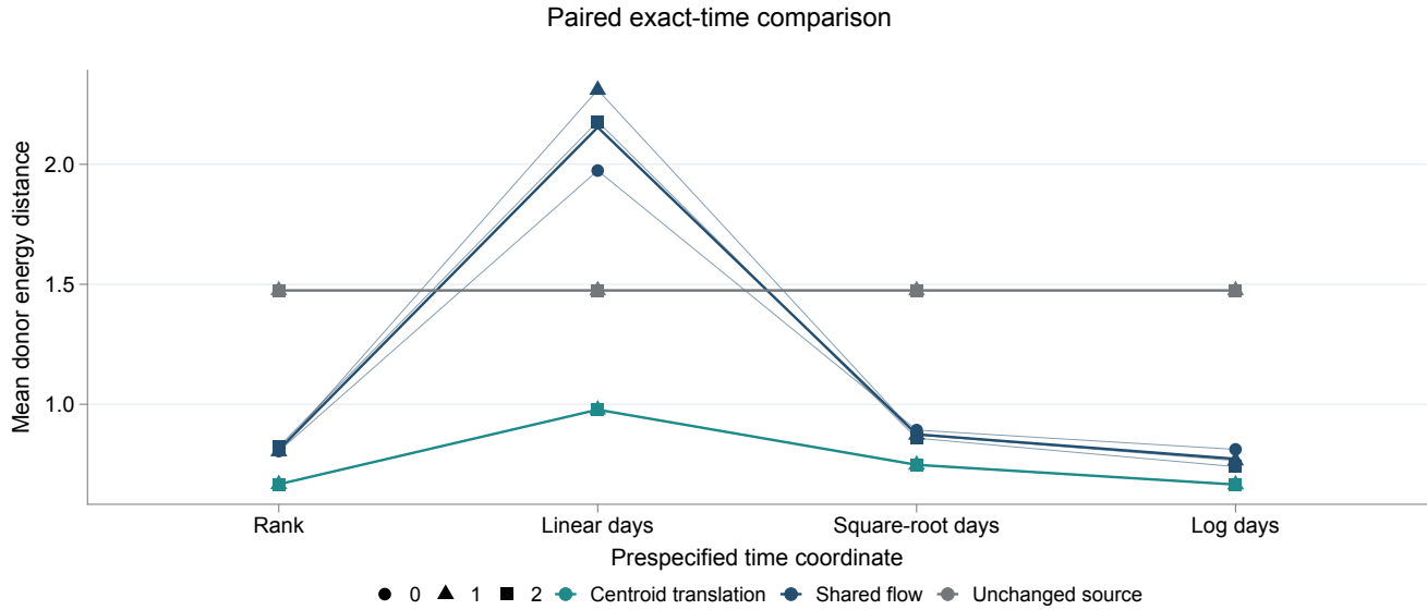
Figure 4. Paired time-coordinate sensitivity under global day-7 holdout in three healthy donors. Twelve fields combine four fixed clocks with seeds 0, 1 and 2, each using 8,000 training steps and batch size 256. Network initialization, endpoint draws and interpolation random draws are paired across clocks within seed. All day-7 cells are excluded from fitting and scaling. Energy distance is evaluated at the exact transformed day-7 time after 50 RK4 steps, using the same source and target rows across clocks and seeds and a 1,200-cell cap per donor. Each point is the equal mean of three donor-specific distances; shapes identify training seeds. Thin lines join the same seed, and thick lines show three-seed means. Colors distinguish shared flow, within-donor centroid translation and unchanged source. The centroid control uses the permitted day-1 and day-30 biopsies, not day-7 expression. Constant baseline points overlap. Connecting categorical clock choices does not depict a biological trajectory, and seed spread is not a biological confidence interval.
