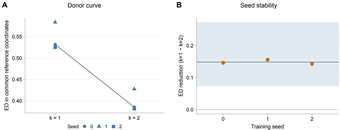
Figure 6. Donor-count comparison in common scoring coordinates. (A) k is the number of training donors. The line joins seed-0 mean held-out errors, 0.5315 at k=1 and 0.3854 at k=2 ; symbols identify seeds 0, 1 and 2. Each model uses only its selected training donors for fitting and normalization. Predictions return to encoder coordinates before scoring under one reference fitted from both non-held donors, fixed across k and seed and excluded from single-donor fitting. At k=1 , two training choices are averaged within held donor before equally weighting the three donors. (B) Points are seed-specific reductions, k=1 minus k=2 . The line is the three-seed mean, 0.1483. Shading is a descriptive percentile 95% range [0.0732, 0.2727] from 4,000 resamples of three donor blocks after seed averaging; it is not an interval for each point. Source and target indices are fixed. The largest configuration-specific seed range is 0.3377. Overlapping training sets limit interval interpretation, and two k values cannot identify a plateau or required cohort size.
