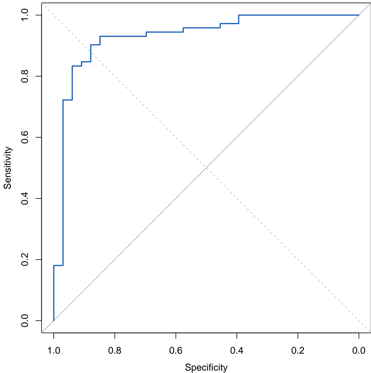
ROC Curve – lassoRF
