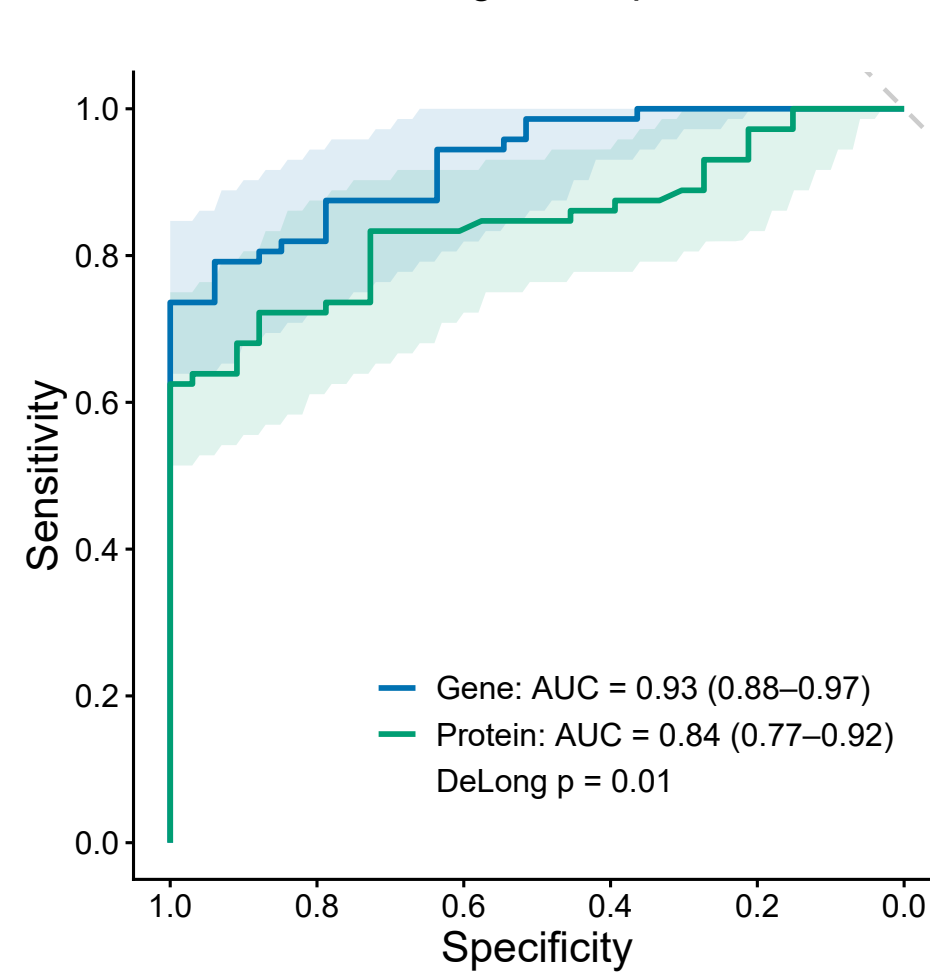
FABP4: gene vs protein
