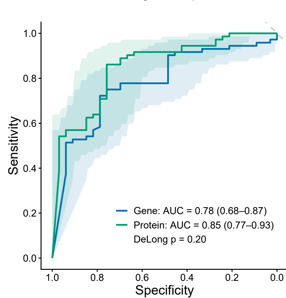
ISG15: gene vs protein
