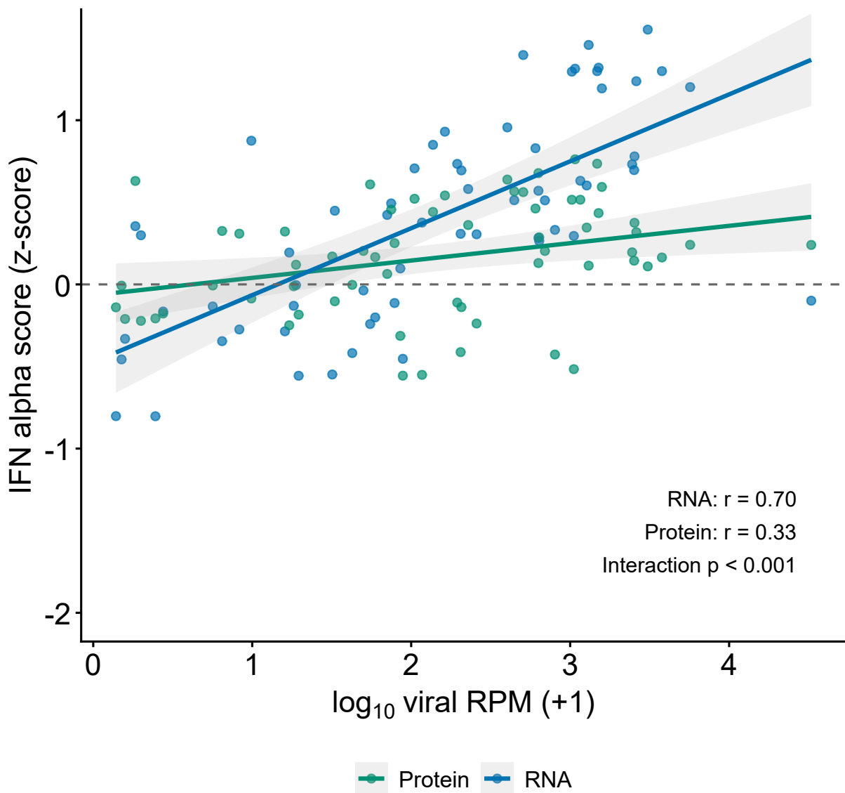
Composite IFN alpha score versus viral abundance
