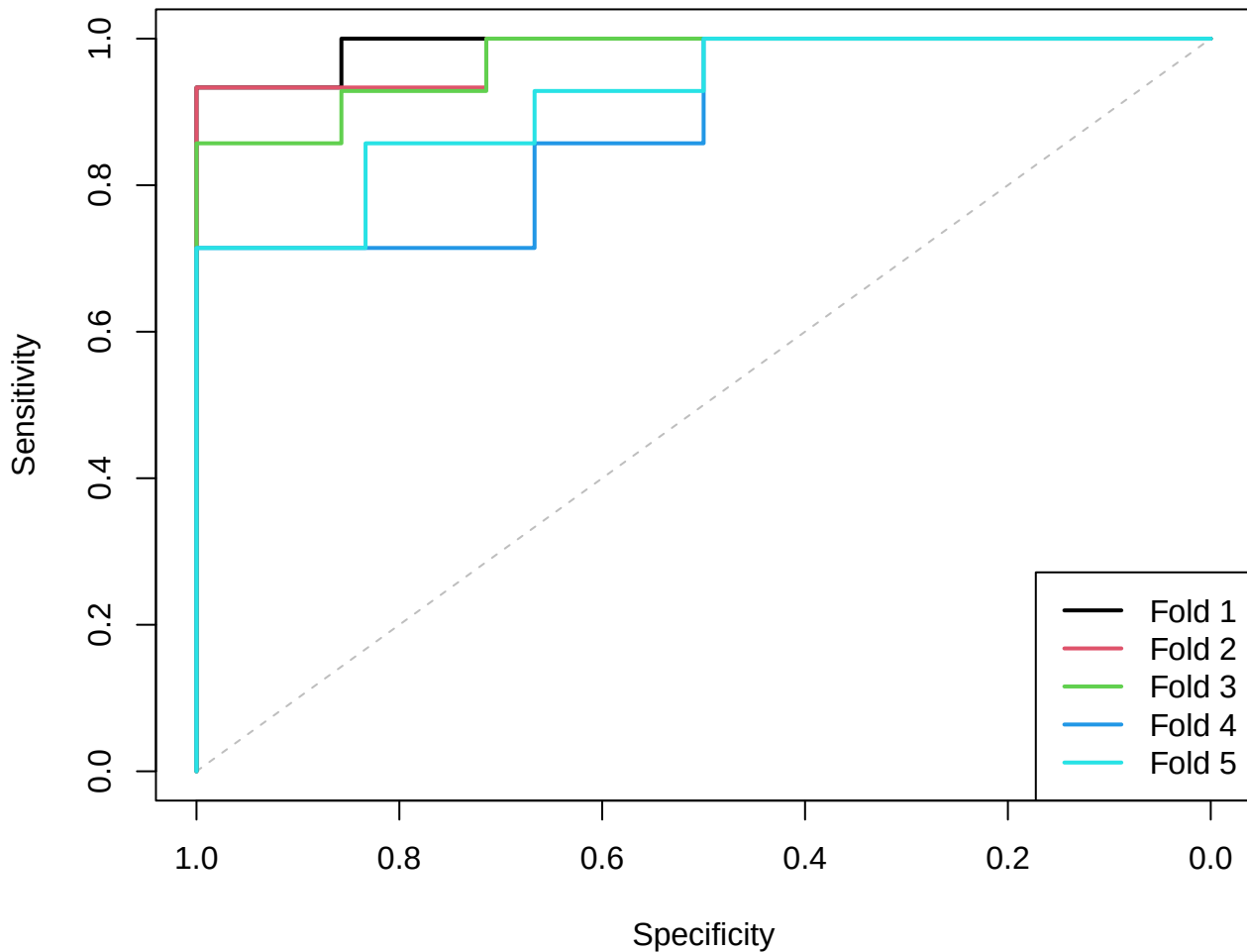
ROC curves by fold
