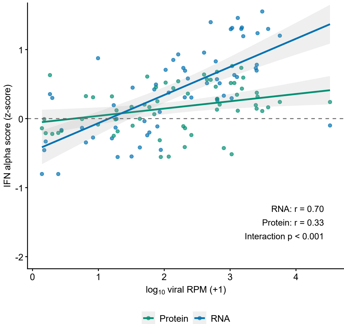
Composite IFN alpha score versus viral abundance
