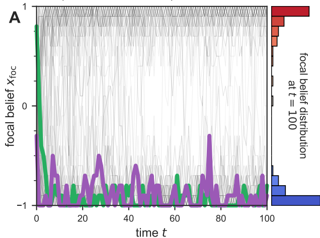
example simulation with adaptive belief networks
