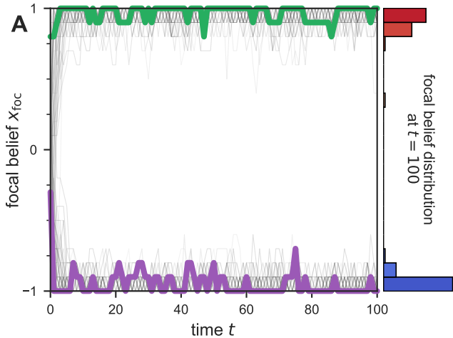
example simulation with static ( \omega_0 = 0.8 ) belief networks
