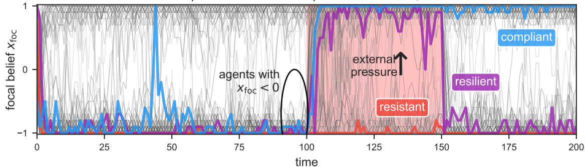
example simulation with adaptive belief network, s = 4
