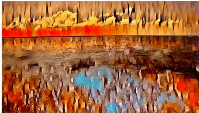
Candy (150%)
