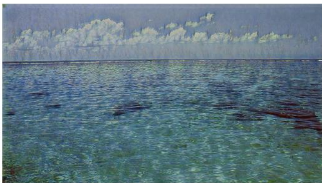
Macke (100%)
