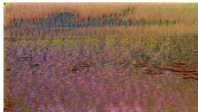
Macke (200%)
