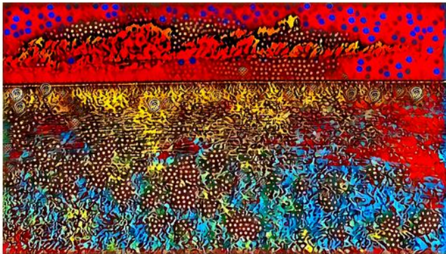
Klee (150%)
