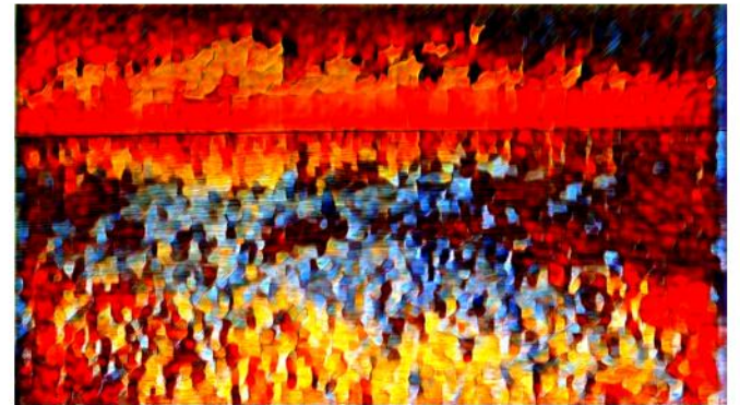
MuchaWorks (200%)
