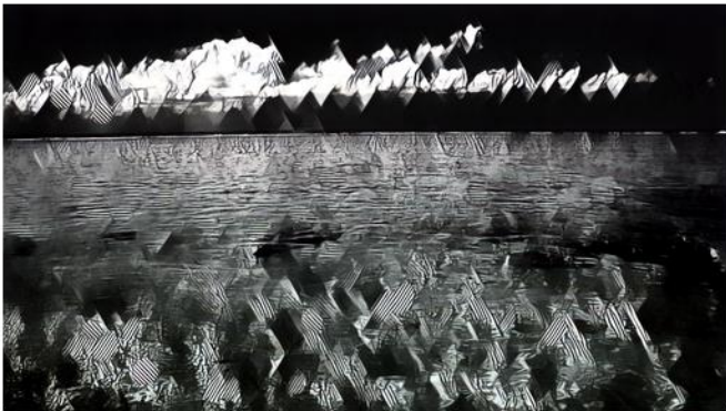
Cézanne (100%)
