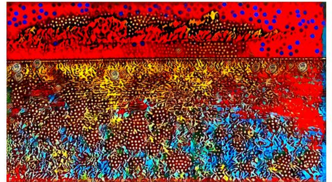
Klee (200%)
