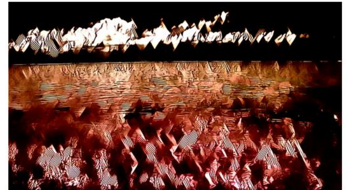
Cézanne (200%)
