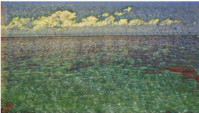
Ukiyo-e (100%)
