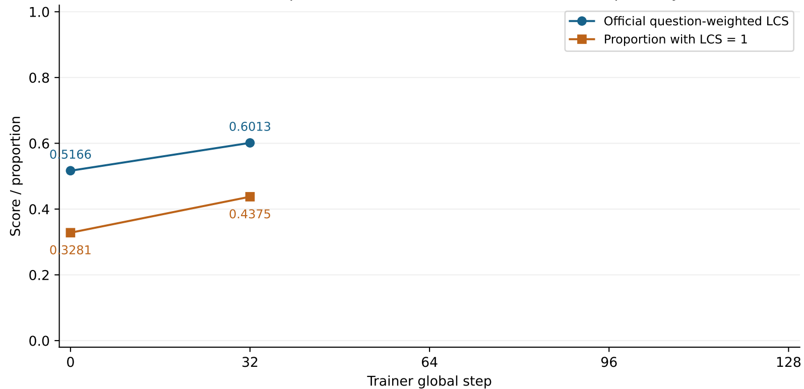
Qwen3-32B / official MemAgent / 35/128 completed steps 64 fixed dev questions; external heldout evaluated separately
