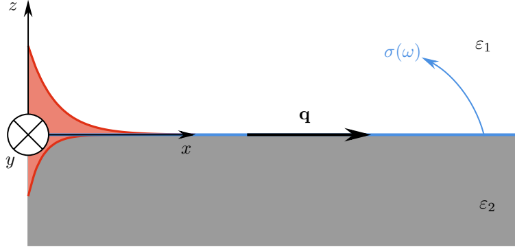
Figure 2.2: Schematic representation of a surface polariton. A polariton with wavevector \mathbf{q} propagating along a 2D material separating two bulk media, medium 1 on top as the cladding material, and medium 2 underneath acting as a substrate. Each medium j = 1, 2 has its own permittivity \varepsilon_j(\omega) , while the 2D material has its own conductivity \sigma(\omega) . The regions shaded in red represent the exponentially decaying amplitude of the polariton along the z direction. In medium 2, assuming it has a higher permittivity than medium 1, the polariton is more confined in comparison with medium 1.
