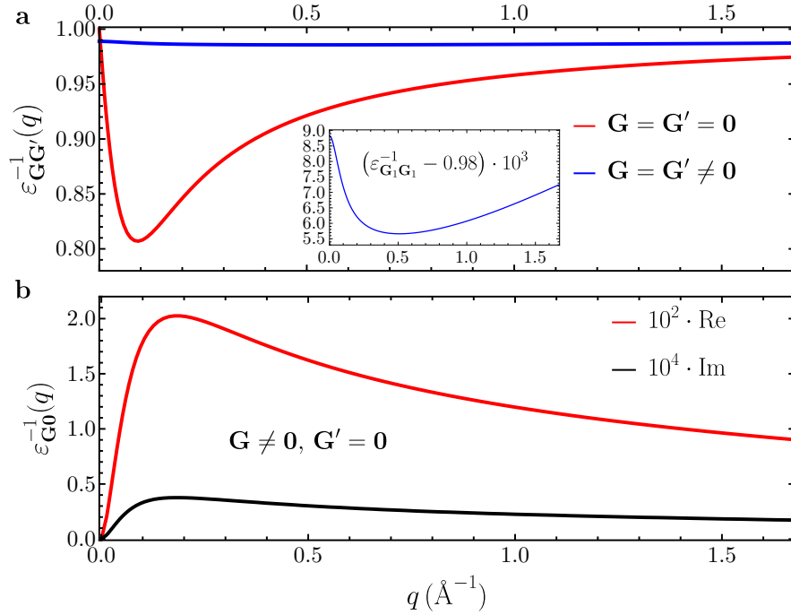
Figure 6.7: Inverse dielectric function matrix elements as a function of momentum. Few inverse dielectric matrix elements \varepsilon_{\mathbf{G}\mathbf{G}'}^{-1} of the inverse dielectric matrix in the BZ for hBN as a function of momentum q . Panel a displays the head element in red and the first diagonal body element \varepsilon_{\mathbf{G}_1\mathbf{G}_1}^{-1} , where the vector \mathbf{G}_1 is the same from Fig. 6.5. The inset in panel a shows the blue curve when we zoom in. This body element is dispersive, but within a much smaller scale than the head element. Panel b displays the real and imaginary parts of the wing element \varepsilon_{\mathbf{G}_1\mathbf{0}}^{-1} in red and black, respectively. This element presents also a q -dependence at a smaller scale than the head element, since both real and imaginary parts are scaled by a power of ten. The momentum \mathbf{q} followed the symmetry line \Gamma - K in the BZ, and the applied cutoff is G_c = 54 \text{ \AA}^{-1} .
