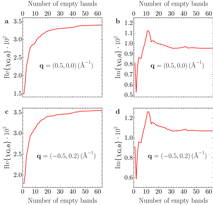
Figure 6.3: Convergence of the polarizability with the number of conduction bands: an wing element. Matrix element \chi_{\mathbf{G}_1,0}^0(\mathbf{q}) of the polarizability, where \mathbf{G}_1 is a primitive vector of the reciprocal lattice, for two different values of momentum \mathbf{q} as a function of included conduction bands for hBN. The left panels display the real part, while the right panels display the imaginary part. The model for hBN is the same as in Fig. 6.2. Herein, \mathbf{G}_1 = (-1.44526, 2.50326) \text{ \AA}^{-1} .
