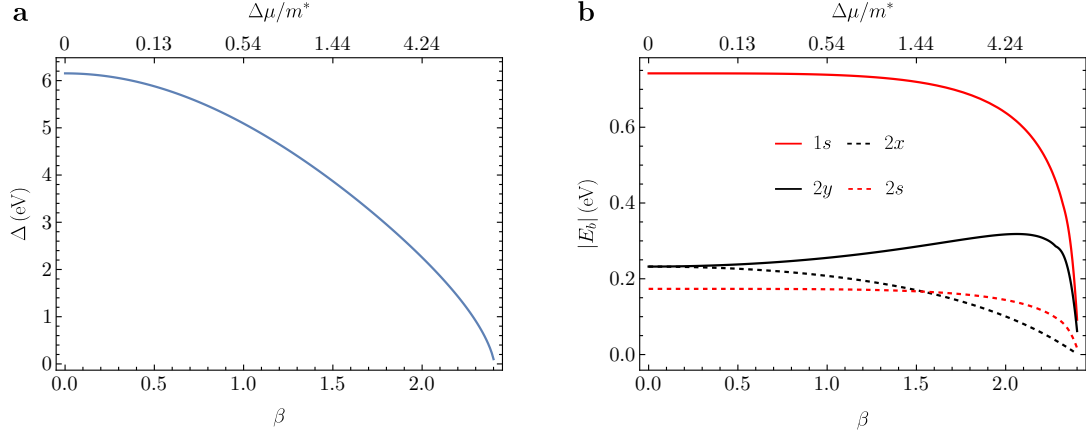
Figure 5.2: Electronic bandgap and excitonic binding energies of a periodically modulated hBN sheet. a Bandgap and b binding energies of the excitonic states as a function of \beta . In b the binding energies of s peaks are represented in red, with a continuous line for the 1s state and with a dashed line for the 2s state, while the p states 2x and 2y are represented with dashed black line and with a continuous black line, respectively. The scale in the top horizontal axis in both plots represent the degree of anisotropy in the dispersion, that we define as \Delta\mu/m^* = (m_y - m_x)/m^* . For hBN, the parameters are [174]: E_g = 3.92 eV, \hbar v_F = 5.06 eV \cdot\text{\AA} , and r_0 = 10 \text{\AA} .
