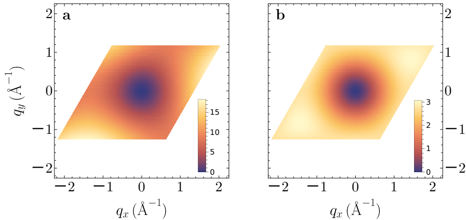
Figure 6.5: Polarizability in the BZ: an wing element. Matrix element \chi_{\mathbf{G}_1\mathbf{0}}^0(\mathbf{q}) of the polarizability in the BZ for hBN. Panel a displays the real part of the polarizability, while panel b displays the imaginary part. The bar legend for the colors are inset. The polarizability is multiplied by 10^2 in both plots.
