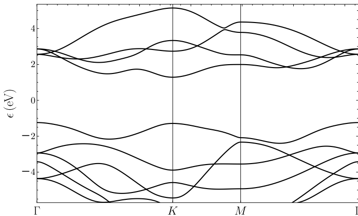
Figure 6.16: Band structure of MoS 2 with a Wannier model. Quasiparticle band structure of monolayer MoS 2 computed through DFT calculations with the QUANTUM ESPRESSO, followed by a Wannierization to change the Hamiltonian to a basis of localized Wannier functions using the WANNIER90 code. The bands were generated with Xatu, in similarity to what we did for hBN in Fig. 6.1. Details of the calculation are in the second paragraph of the previous page.
