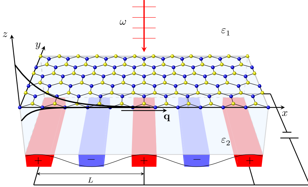
Figure 5.1: A single hBN monolayer electrostatically modulated. A hBN monolayer over a substrate, subjected to an external periodic potential with period L along the x -direction, under a time-periodic drive of a linearly polarized optical field.
