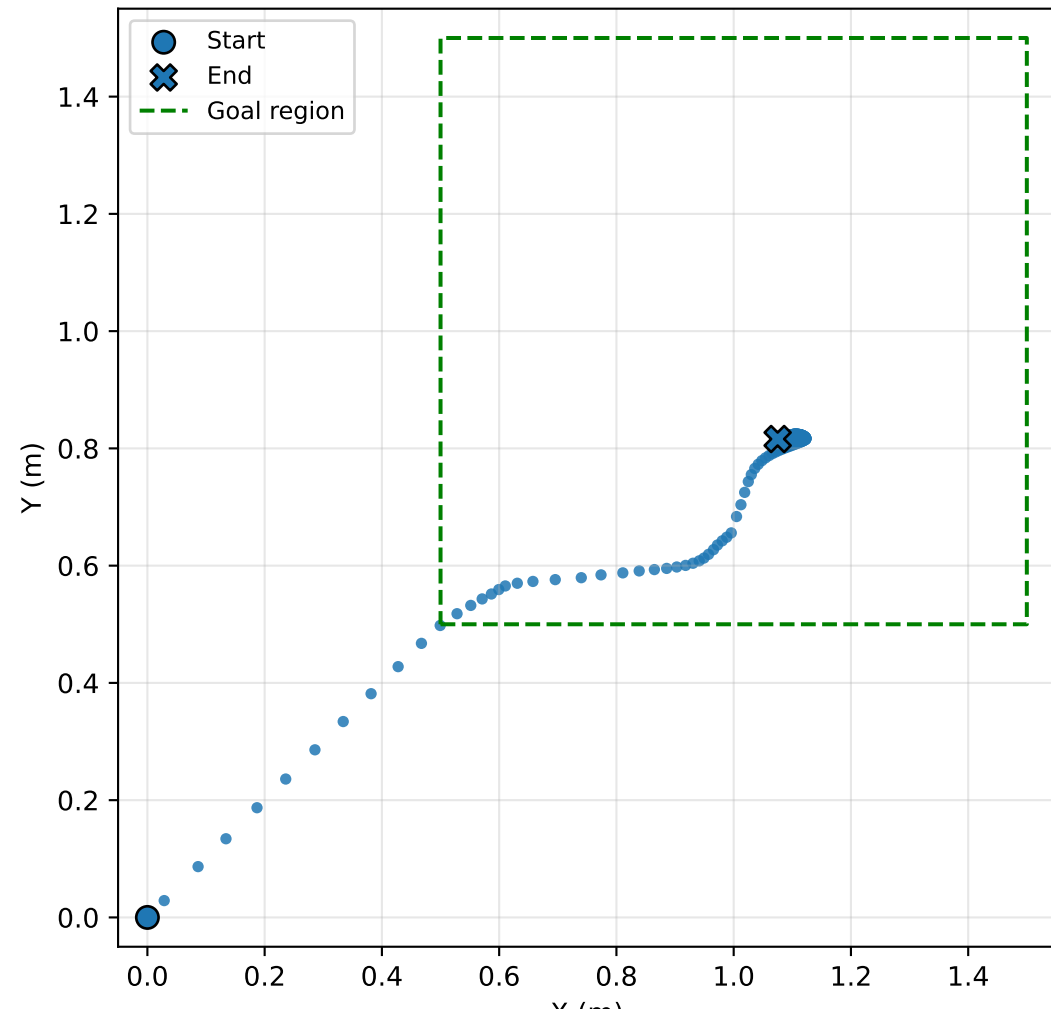
Top view (XY plane, looking -Z)
