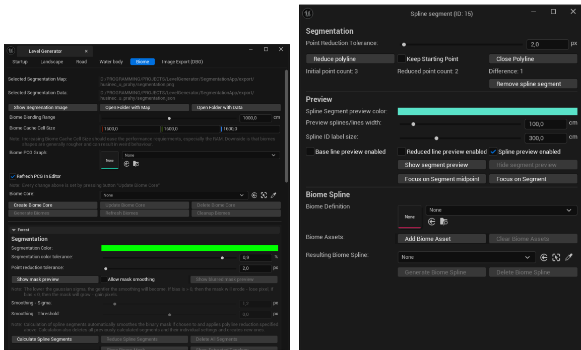
(a) Biome page with two segmentation regions of type BIOME: Forest and Quarry.
