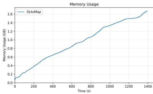
(a) Memory consumption over the duration of dataset experiment 0102
