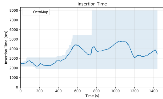
(b) Point cloud insertion time over the duration of dataset experiment 0201
