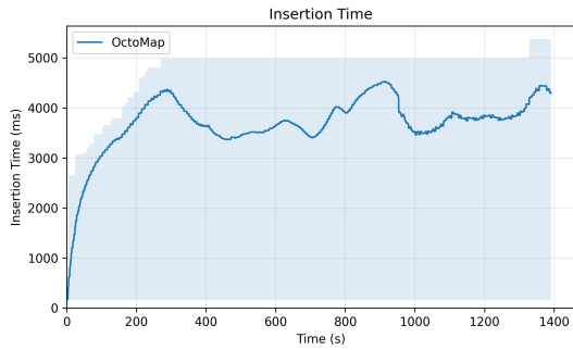
(a) Point cloud insertion time over the duration of dataset experiment 0102
