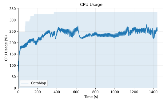
(b) CPU usage over the duration of dataset experiment 0201
