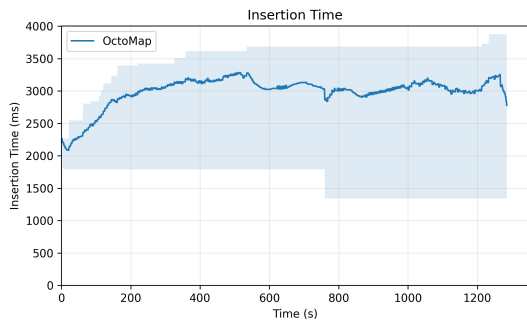
(c) Point cloud insertion time over the duration of dataset experiment 0302
