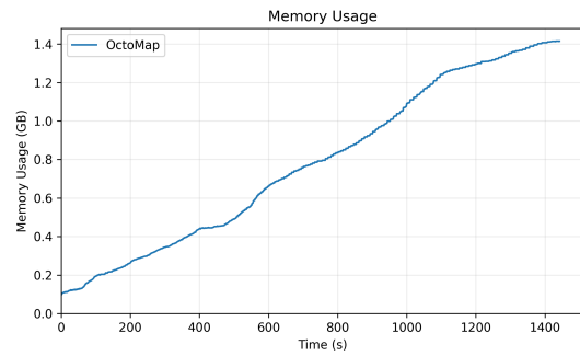
(b) Memory consumption over the duration of dataset experiment 0201
