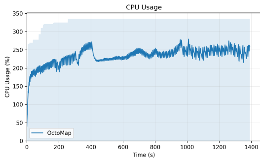
(a) CPU usage over the duration of dataset experiment 0102
