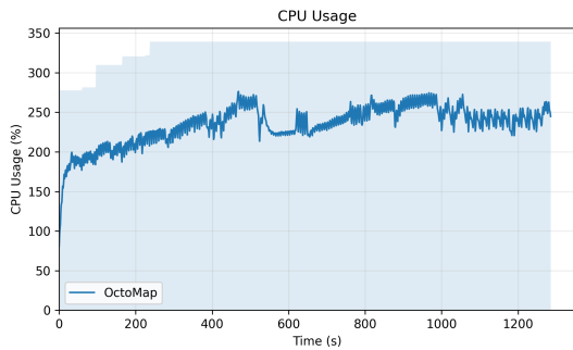
(c) CPU usage over the duration of dataset experiment 0302
