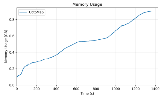
(d) Memory consumption over the duration of dataset experiment 0402
