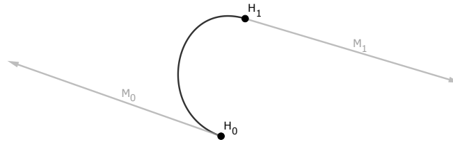
Figure 2.3: Example of Hermite spline constructed from two points and two tangent vectors.
