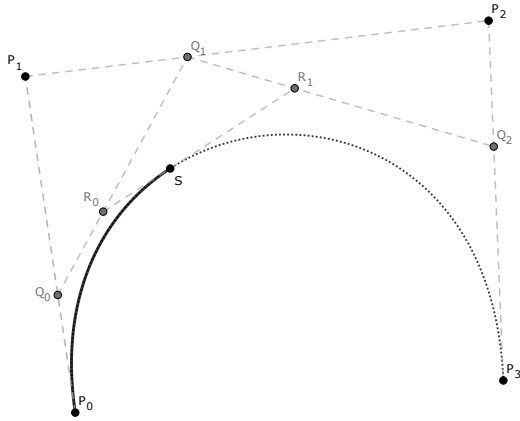
(a) Left spline subdivision.
