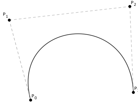
Figure 2.2: Example of cubic Bézier curve constructed from four control points.
