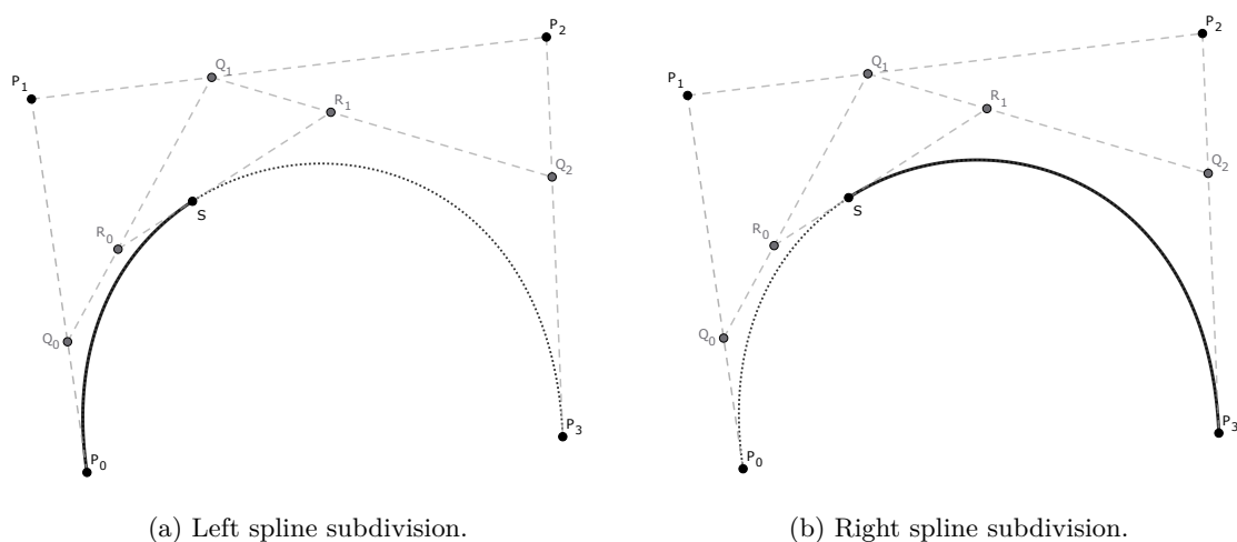
Figure 2.13: Example of subdividing Bézier curve using de Casteljau algorithm for u = 0.35 , the left subdivision (a) and the right subdivision (b).
