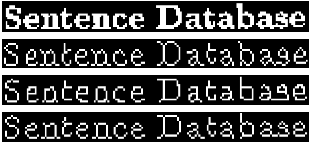
Figure 2.4: Comparison between different skeletonization algorithms. Image was taken from [8]. From top to bottom: (a) Original pattern, (b) Guo–Hall algorithm, (c) Zhang–Suen algorithm, (d) Jain–Kumar algorithm.
