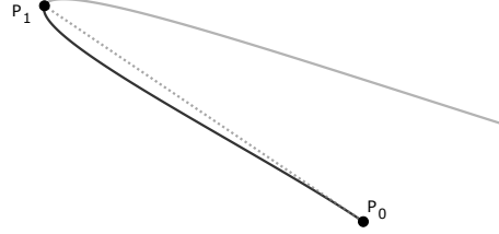
Figure 2.7: Example of Catmull–Rom endpoint extension sharp curve.
