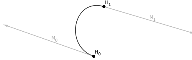
Figure 2.4: Example of Hermite spline constructed from two points and two tangent vectors.
