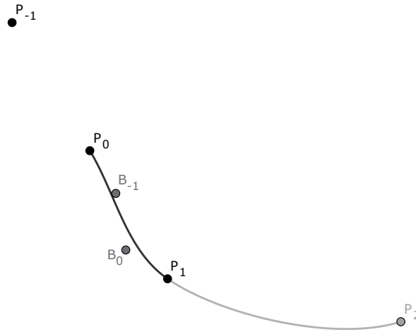
Figure 2.6: Example of Catmull–Rom endpoint extension.
