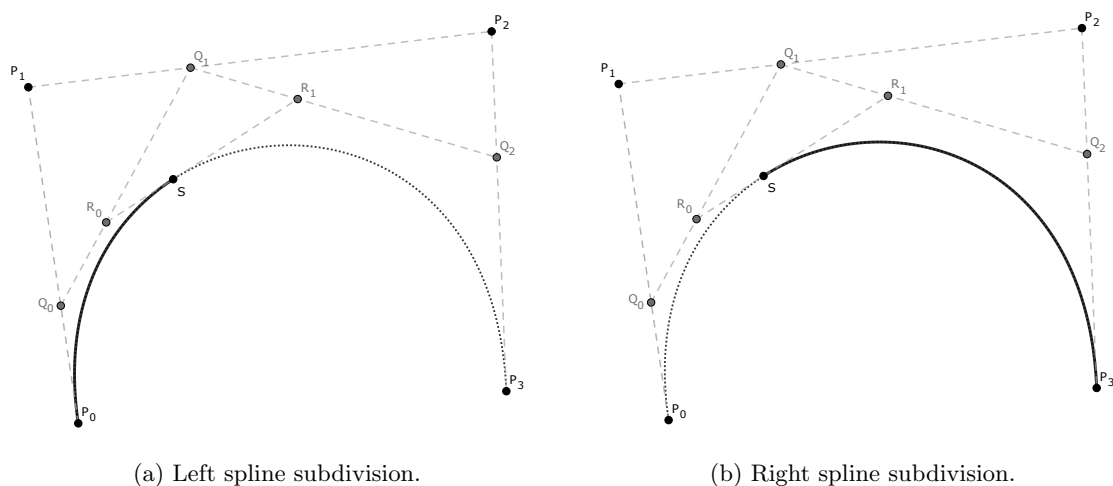
Figure 2.9: Example of subdividing Bézier curve using de Casteljau algorithm for u = 0.35 , the left subdivision (a) and the right subdivision (b).
