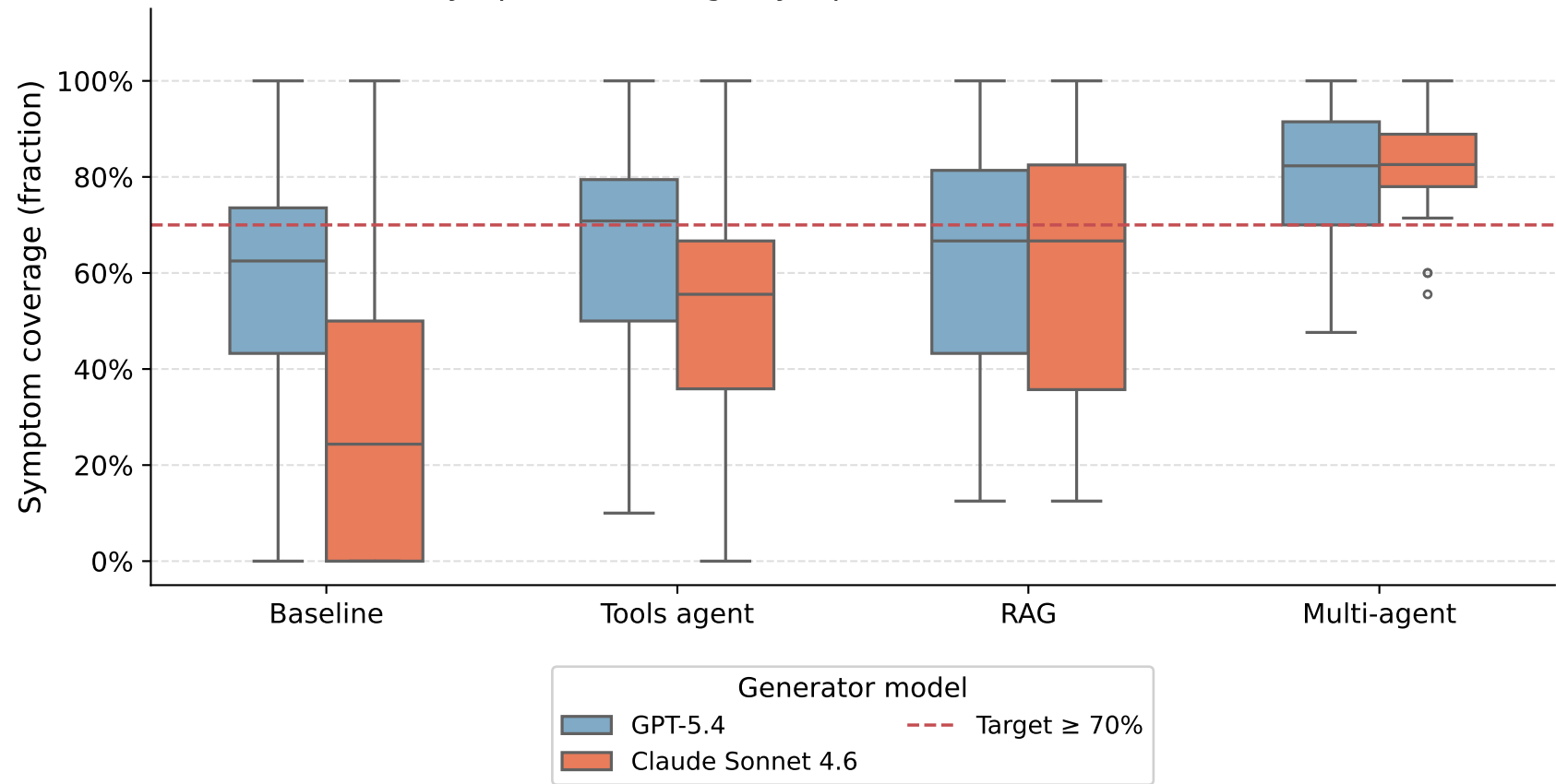
Symptom Coverage by Pipeline and Generator Model
