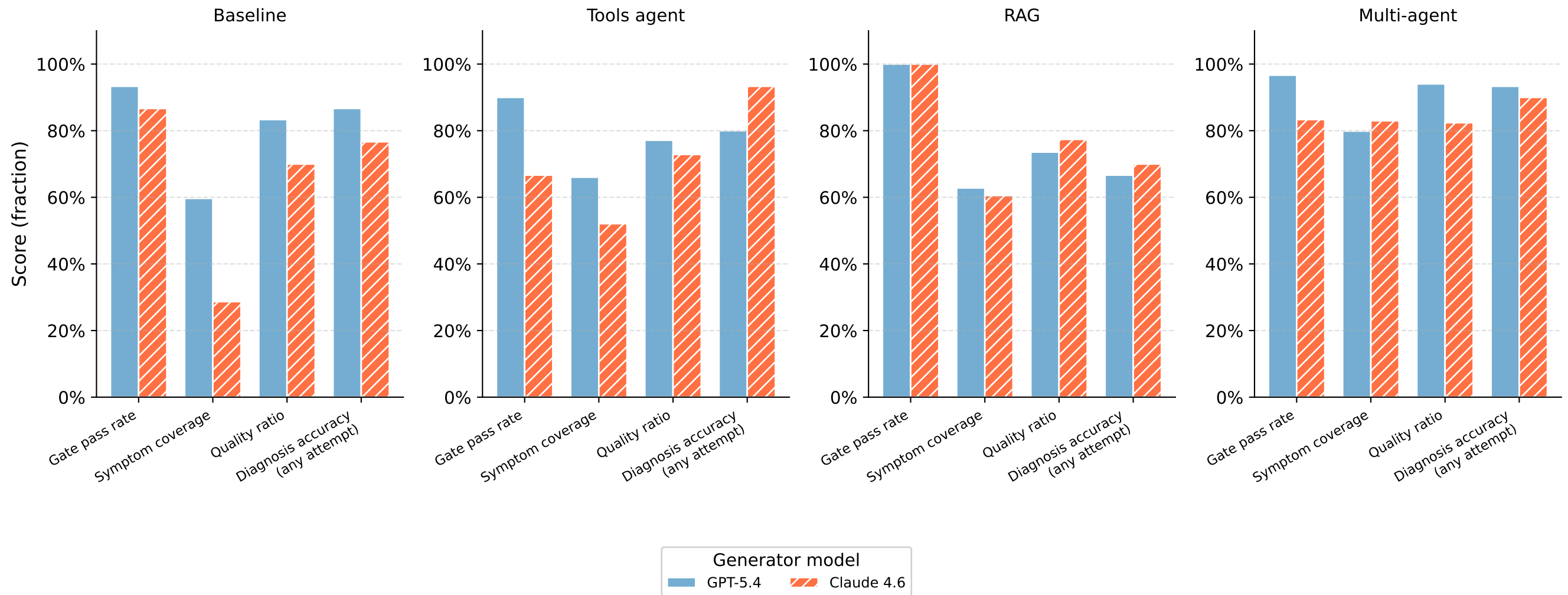
Generator Model Comparison (GPT-5.4 vs Claude Sonnet 4.6) per Pipeline
