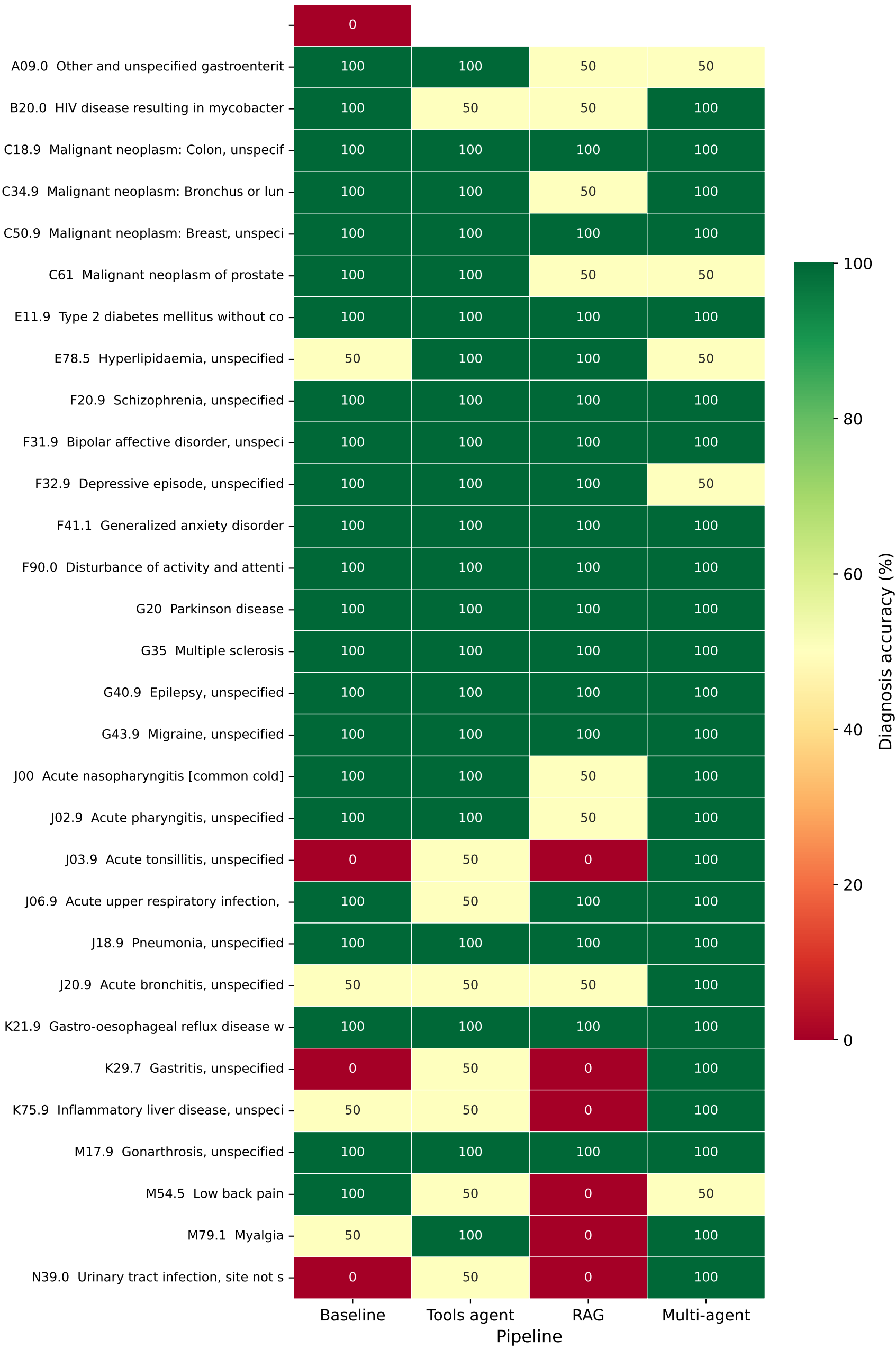
Diagnosis Accuracy (%) per ICD-10 Code and Pipeline (averaged over both generator models and all attempts)
