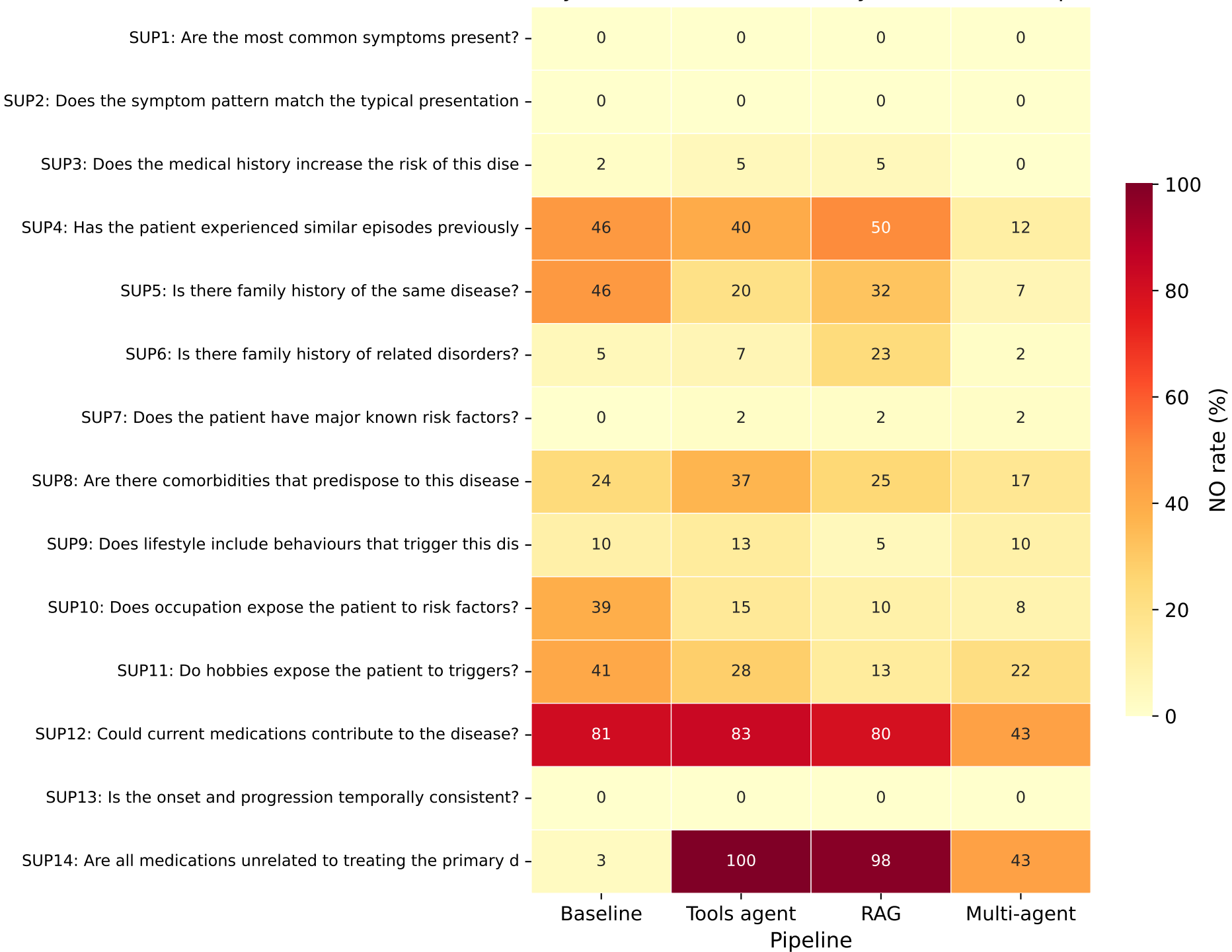
Quality Question NO Rate (%) by Question and Pipeline
