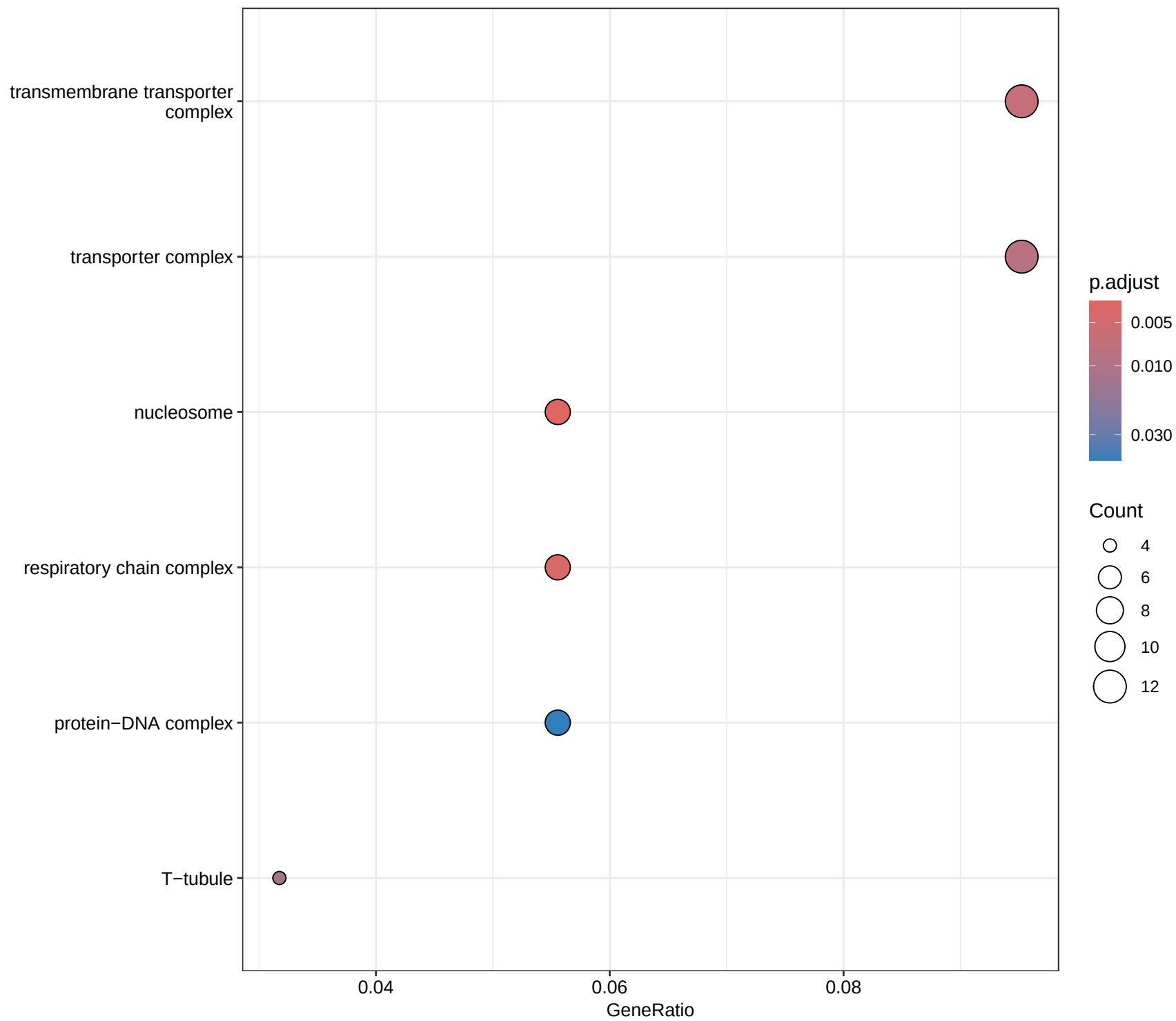
GO-CC ORA — All significant DEGs
