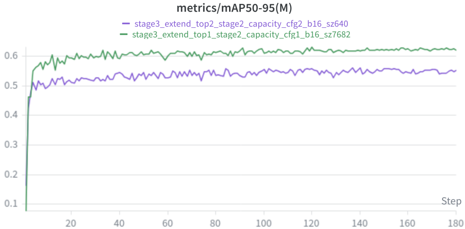
Figure 4.3: Stage 3 validation mask \text{mAP}_{50:95} for the two refinement branches.
