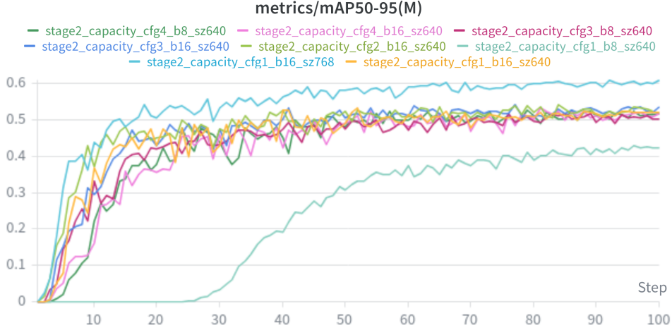
Figure 4.2: Validation mask \text{mAP}_{50:95} for the successful unique Stage 2 capacity-tuning configurations.
