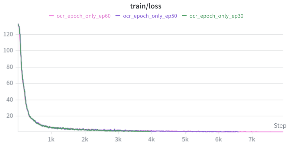
Figure 4.8: Stage 1 OCR training loss for the epoch-selection runs. Most of the optimization progress occurs before the 50-epoch mark, which supports the decision to use 50 epochs for the subsequent optimizer sweep.
