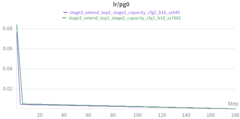
Figure 4.5: Stage 3 learning-rate schedule ( lr/pg0 ) for the two corrected refinement branches. Both runs follow essentially the same decay schedule, so the difference in final accuracy cannot be attributed to different learning-rate behavior.
