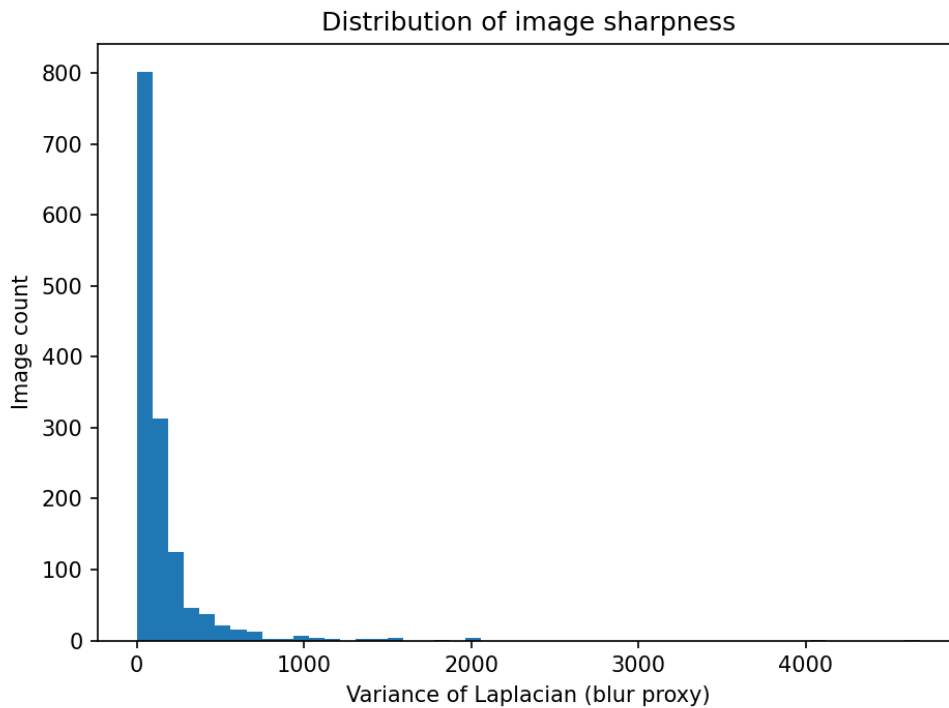
Figure B.1: Distribution of the blur indicator computed from the training images. The spread confirms that the dataset contains both softer and sharper images instead of a single tightly controlled acquisition setting.
