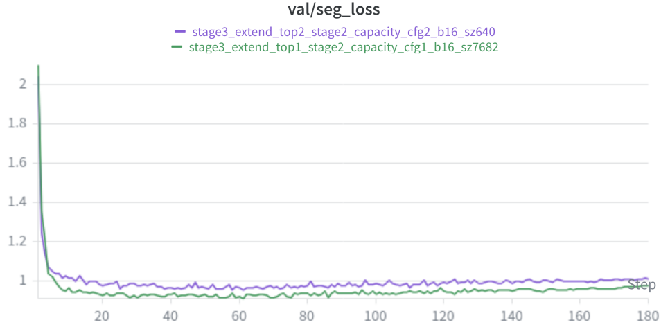
Figure 4.4: Stage 3 validation segmentation loss for the two corrected refinement branches. The branch initialized from the stronger Stage 2 configuration maintains the lower validation loss.
