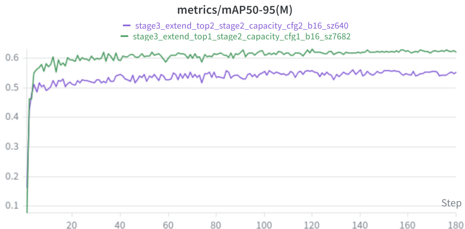
Figure 4.3: Stage 3 validation mask mAP_{50:95} for refinement from the best Stage 2 768-pixel configuration and the second-best unique 640-pixel configuration. The 768-pixel branch remains clearly superior throughout training.
