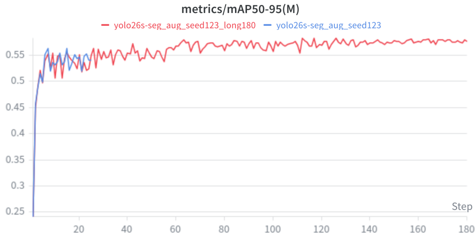
Figure 4.6: Validation mask mAP 50:95 for the two YOLO26 training runs. The longer 180-epoch run improved over the shorter run, but the resulting model still did not surpass the YOLOv8 baseline on the held-out test set.
