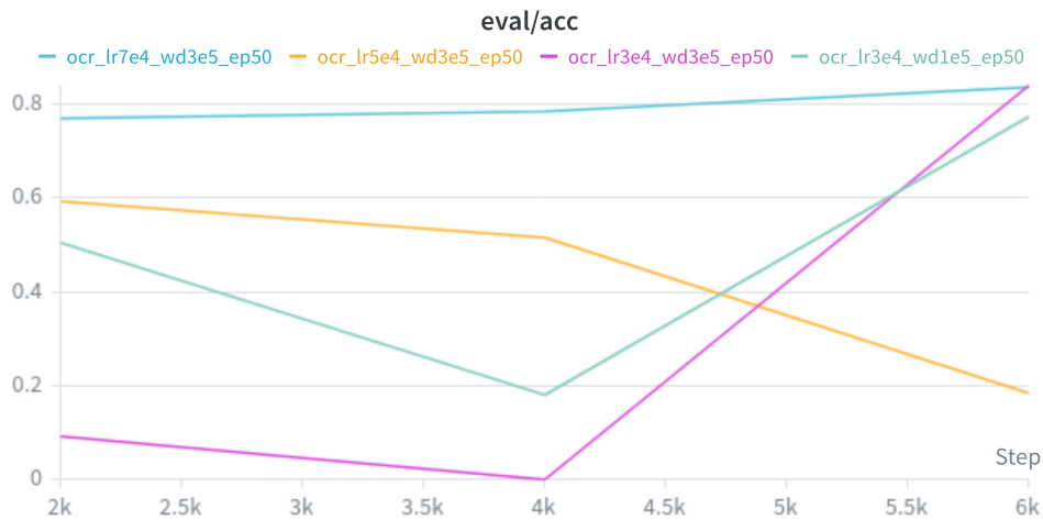
Figure 4.9: Stage 2 OCR evaluation accuracy for the learning-rate and weight-decay sweep. The configuration with learning rate 3 \times 10^{-4} and weight decay 3 \times 10^{-5} achieved the best validation accuracy.
