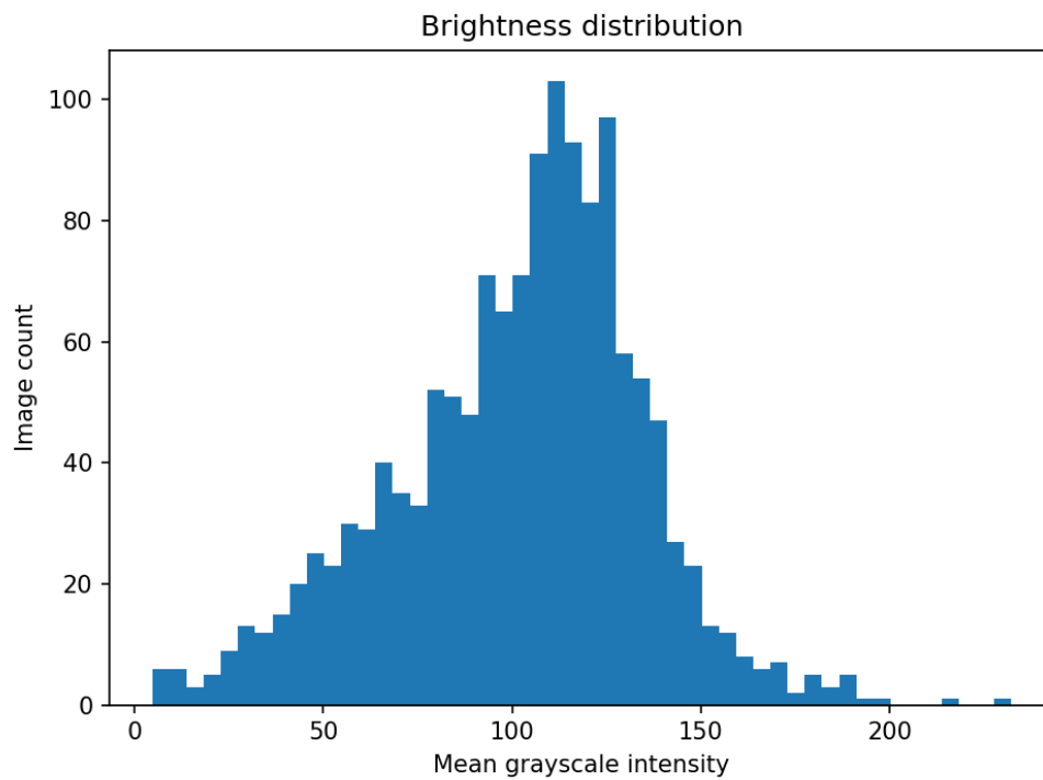
Figure B.2: Distribution of the mean grayscale intensity across the training images. The dataset spans a broad but still usable range of illumination conditions.
