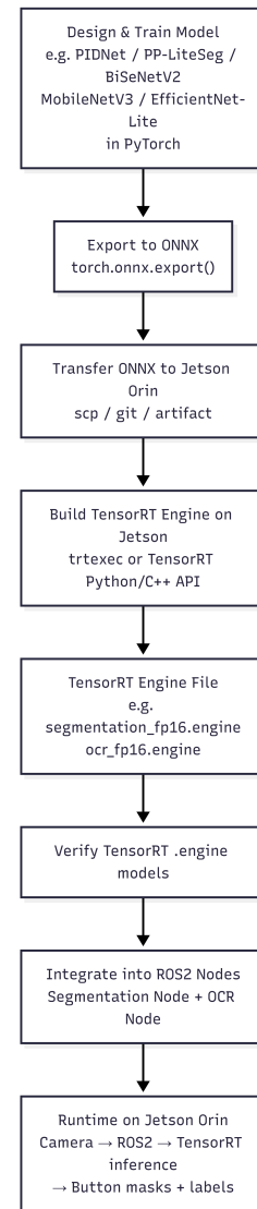
Figure 3.5: Deployment and optimization workflow for models on NVIDIA Jetson Orin using Open Neural Network Exchange (ONNX) and TensorRT (TensorRT).
