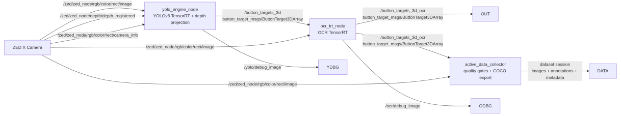
Figure 3.6: ROS 2 runtime architecture used for deployment. The ZED X camera provides image, depth, and camera calibration topics to the YOLO node. The OCR node enriches the geometric targets with text labels, and the active data collector stores accepted deployment samples for later retraining.
