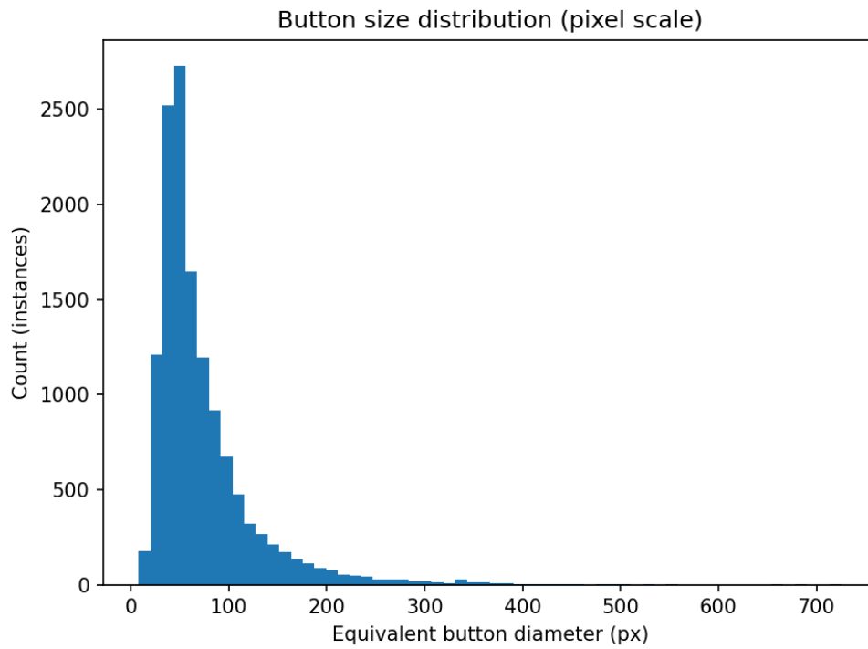
Figure C.1: Distribution of the equivalent button diameter measured from the annotated instances. The x-axis shows the estimated button diameter in pixels, while the y-axis shows the number of annotated button instances in each histogram bin. This figure directly supports the button-size summary values reported in Chapter 4.
