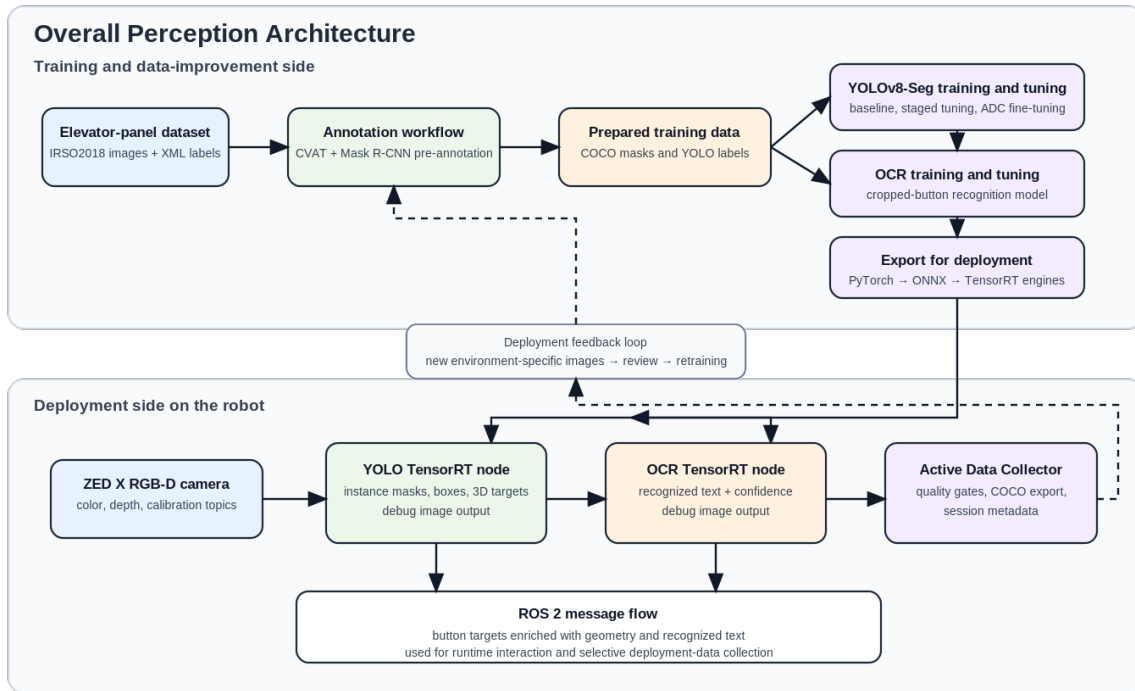
Figure 3.1: Overall workflow-and-architecture overview of the proposed perception system. The figure links dataset preparation, semi-automatic annotation, model training, deployment on the robot, and the feedback path created by the ADC. The detailed training-side annotation workflow is shown later in Figure 3.3, and the deployed runtime pipeline is shown in Figure 3.6.
