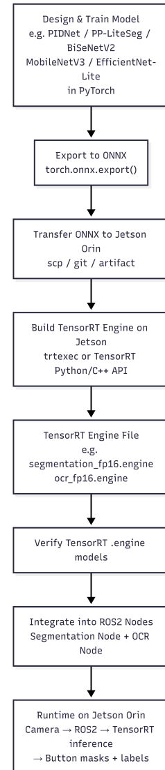
Figure 3.5: Jetson deployment workflow.
