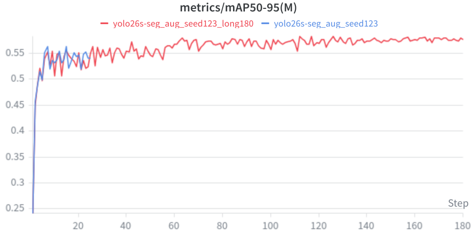
Figure A.3: Validation mask mAP_{50:95} for the two YOLO26 training runs.
