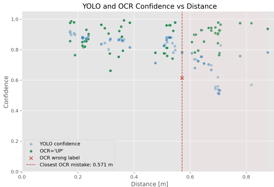
Figure C.1: Supplementary single-button R29 replay plot showing YOLO confidence, OCR confidence, and the distances at which OCR stopped reading the UP button correctly.
