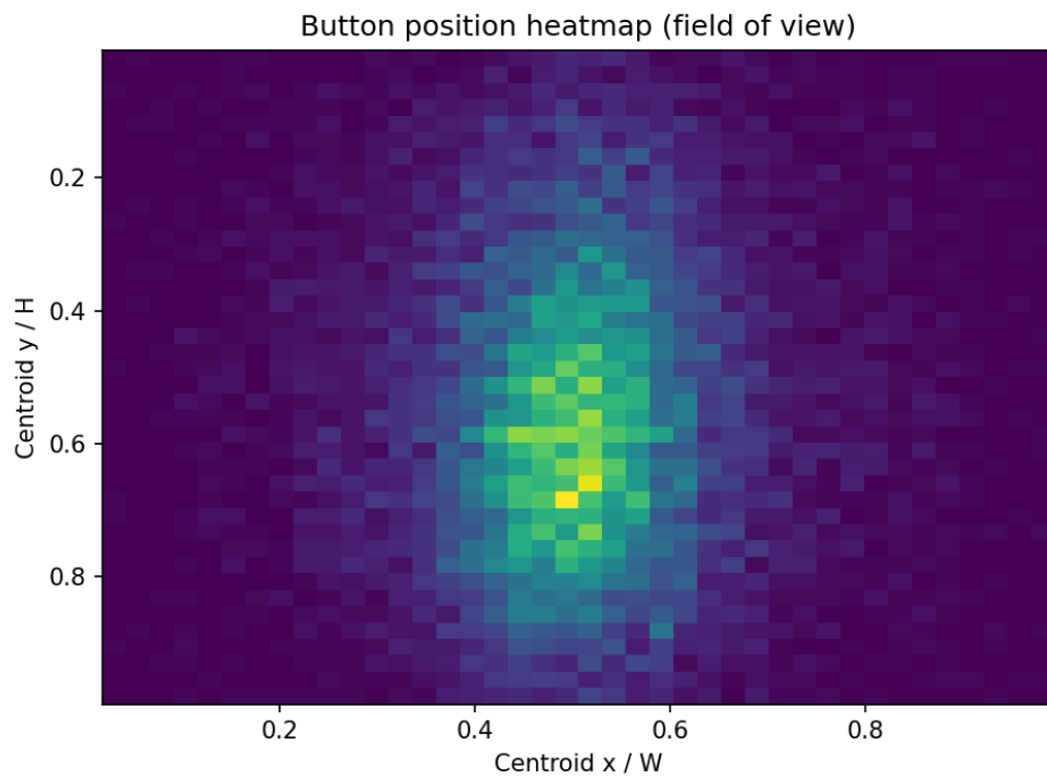
Figure D.3: Heatmap of annotated button-centroid locations in normalized image coordinates. The x-axis shows the horizontal centroid position normalized by image width, with 0 at the left image border and 1 at the right border. The y-axis shows the vertical centroid position normalized by image height, with 0 at the top of the image and 1 at the bottom. The color intensity represents how many annotated button instances fall into each two-dimensional bin.
