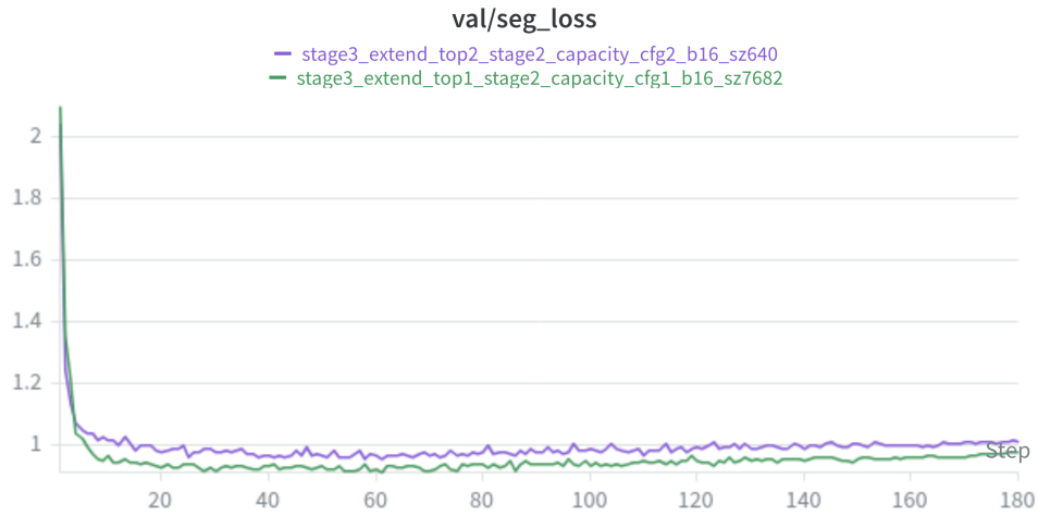
Figure A.2: Stage 3 validation segmentation loss for the two refinement branches.
