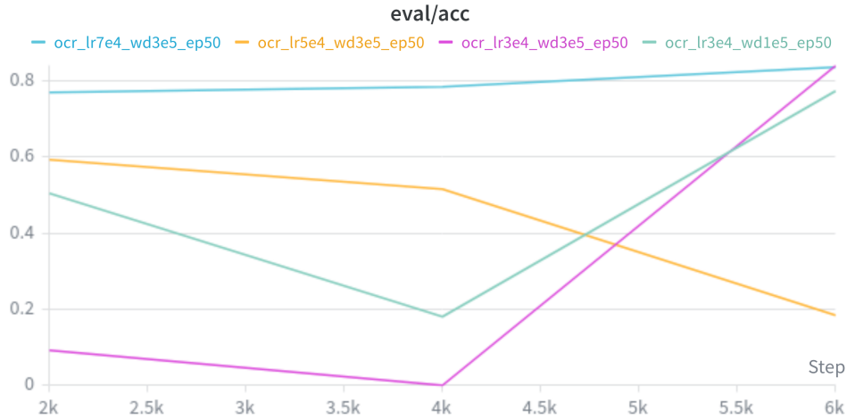
Figure 4.6: Stage 2 OCR validation accuracy for the learning-rate and weight-decay sweep.
