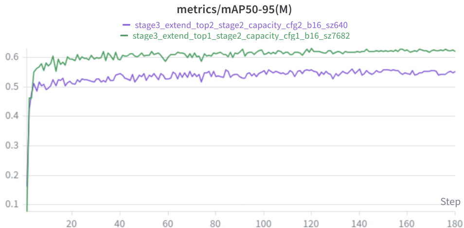
Figure 4.2: Stage 3 validation mask mAP 50:95 for the two refinement branches.
