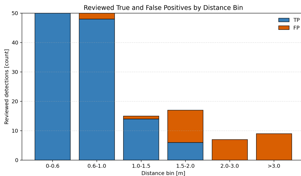
Figure C.2: Reviewed true and false positive detections by distance bin on the longer university replay run. Close-range bins were sampled, while the longer-distance bins were reviewed exhaustively.
