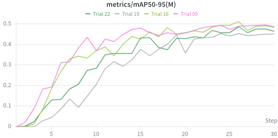
Figure A.1: Validation mask mAP 50:95 for the successful Stage 1 hyperparameter trials.
