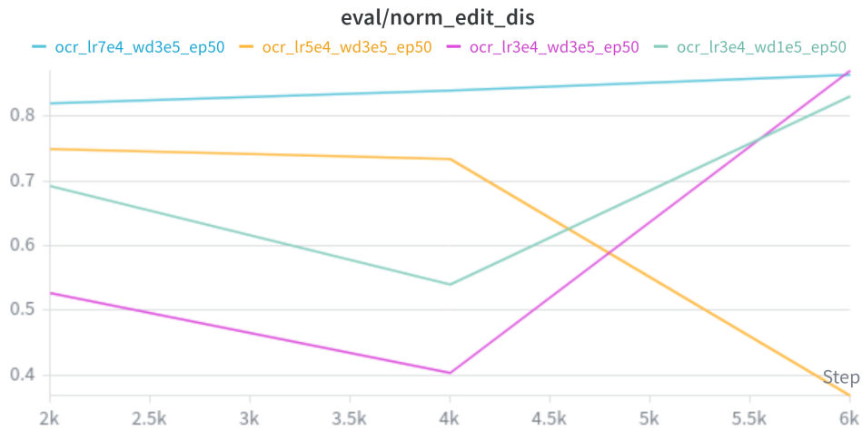
Figure A.4: Stage 2 OCR normalized edit distance for the learning-rate and weight-decay sweep.
