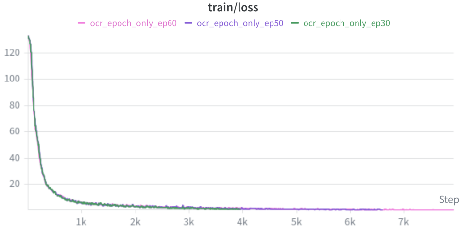
Figure 4.5: Stage 1 OCR training loss for the epoch-selection runs.
