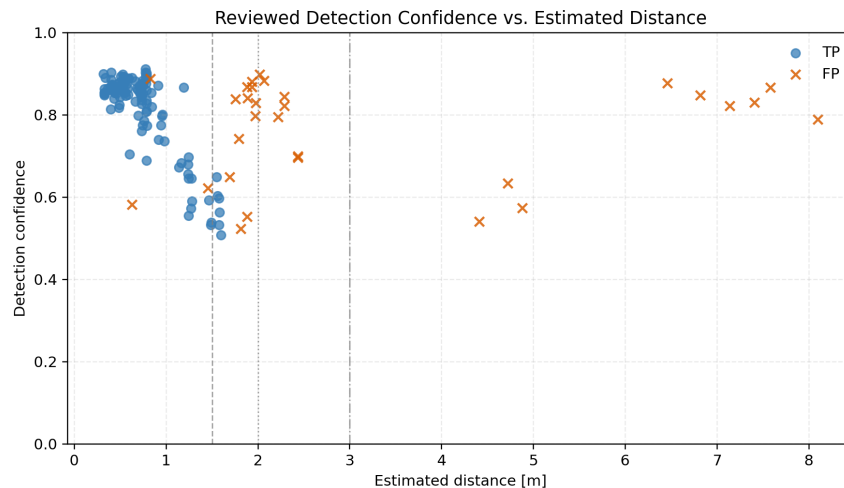
Figure 4.8: Reviewed YOLO detection confidence versus estimated distance on a realistic university elevator replay run. True and false detections were manually reviewed after replay.
