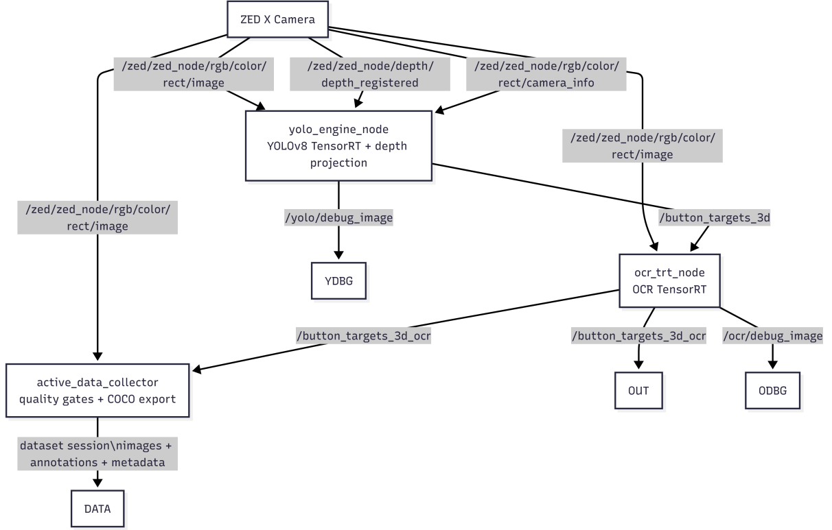
Figure 3.6: Deployed ROS runtime architecture with the ZED X RGB-D camera, YOLO node, OCR node, and active data collector. Gray boxes indicate ROS topics, and white boxes indicate nodes or terminal outputs.
