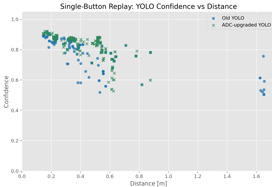
Figure 4.4: Controlled single-button replay result: confidence versus estimated distance for the baseline and ADC-fine-tuned YOLO models.
