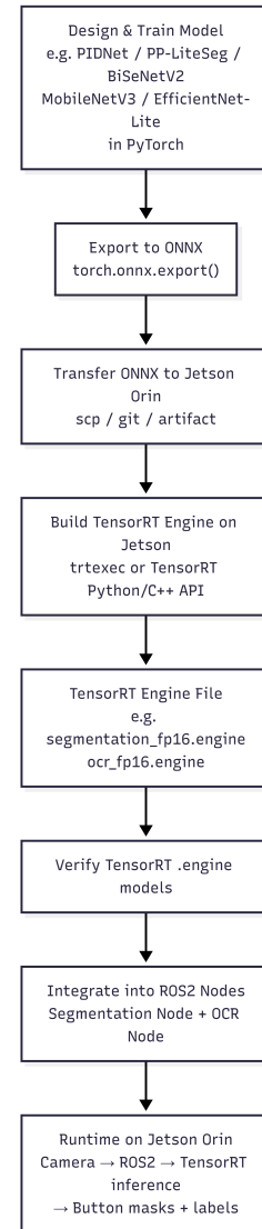
Figure 3.5: Jetson deployment workflow.
