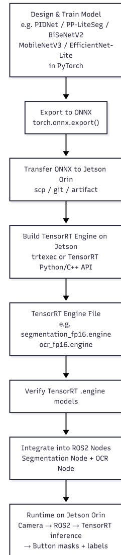
Figure 3.5: Jetson deployment workflow via Open Neural Network Exchange (ONNX) and TensorRT (TensorRT).
