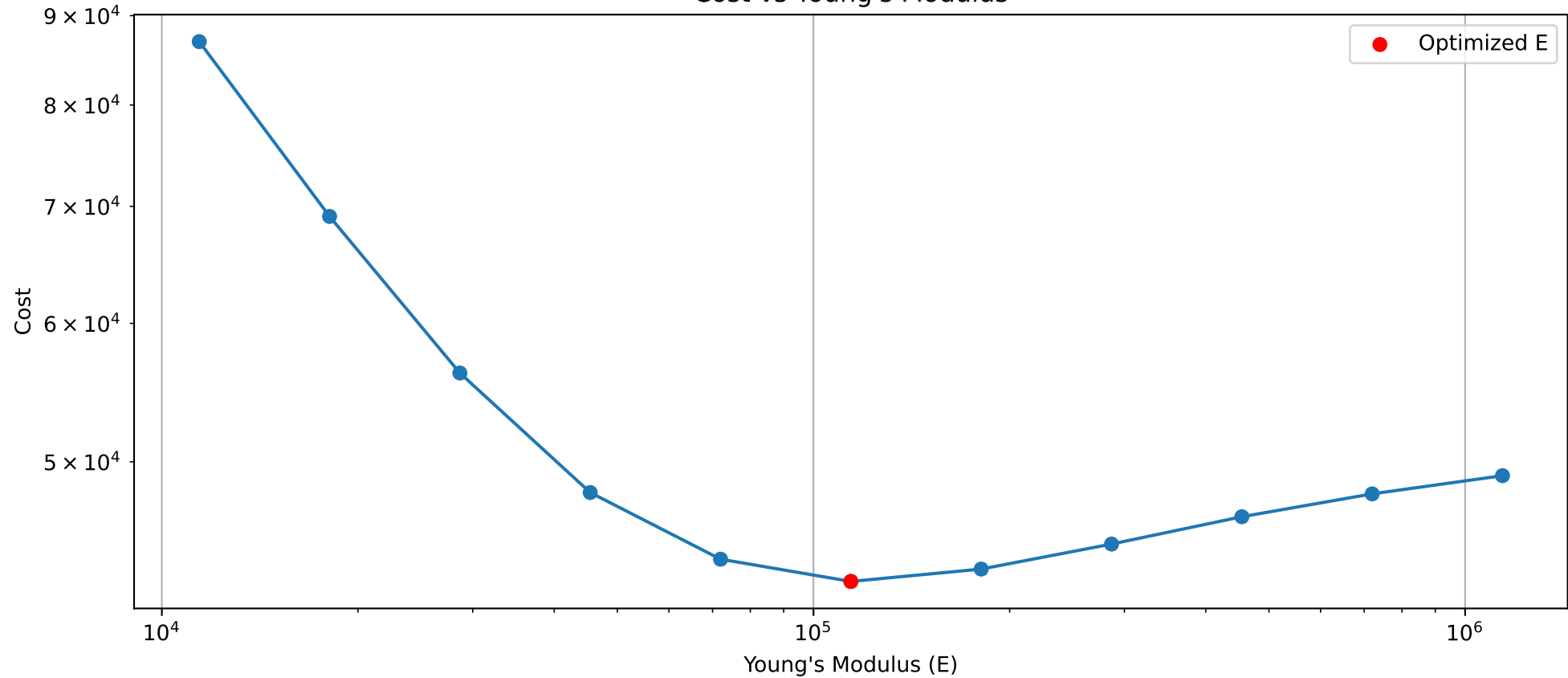
Cost vs Young's Modulus
