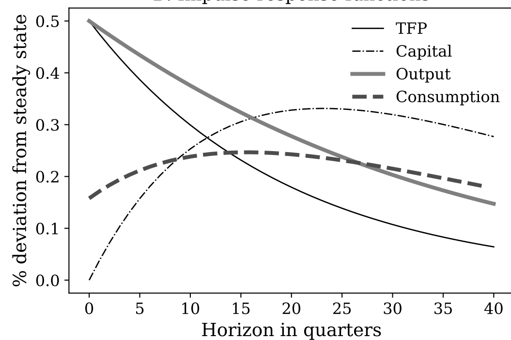
B. Impulse response functions
