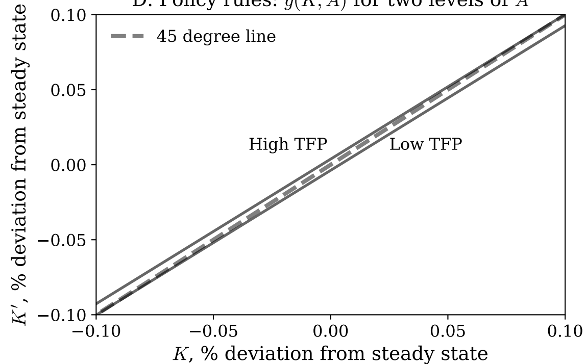
D. Policy rules: g(K, A) for two levels of A
