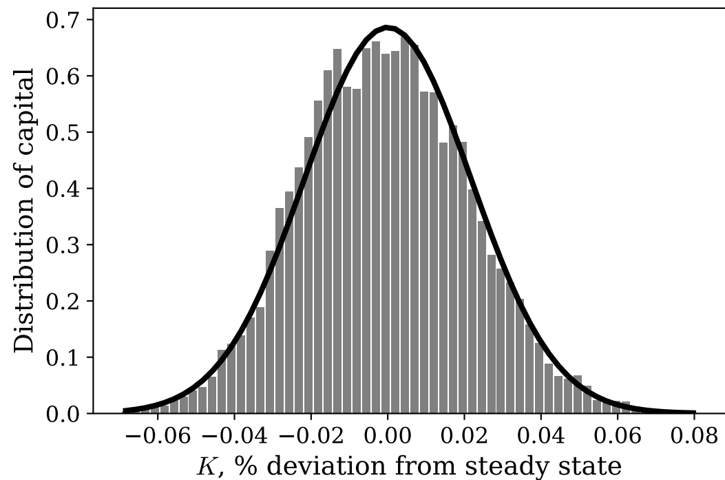
C. Distribution of K
