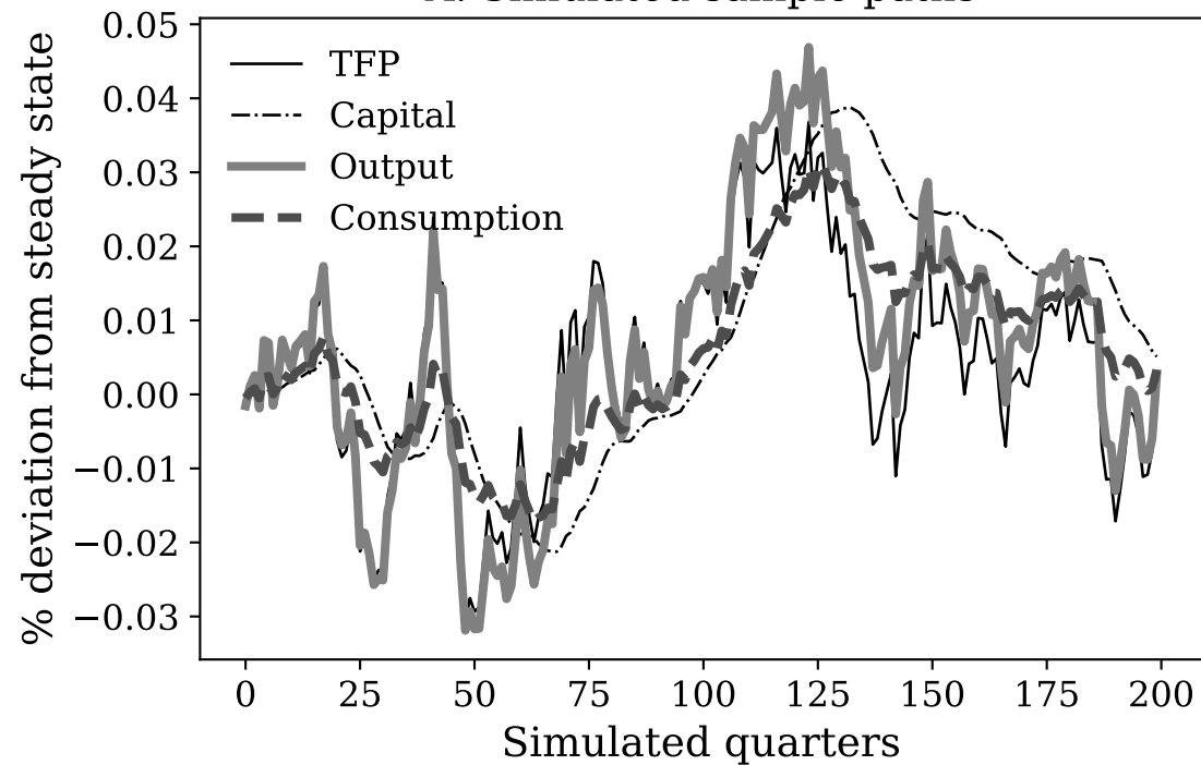
A. Simulated sample paths
